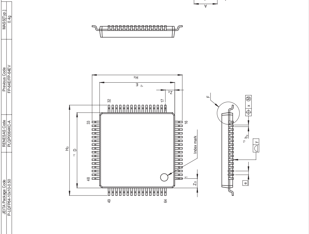
Figure D.1 FP-64E Package Dimensions
