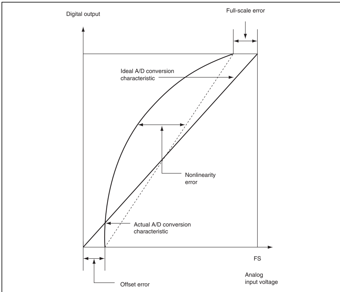
Figure 17.5 A/D Conversion Accuracy Definitions (2)
