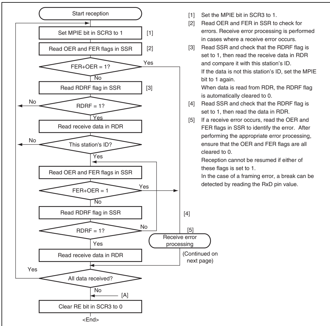
Figure 15.17 Sample Multiprocessor Serial Reception Flowchart (1)
