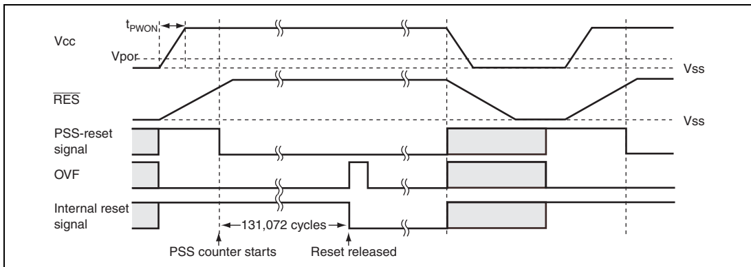
Figure 18.2 Operational Timing of Power-On Reset Circuit
