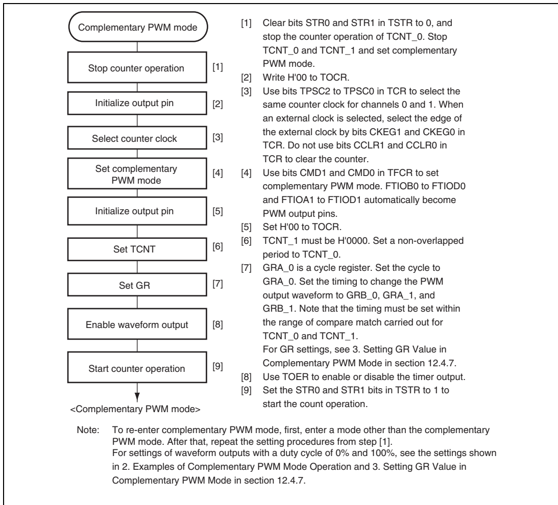
Figure 12.29 Example of Complementary PWM Mode Setting Procedure
