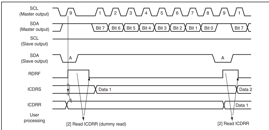
Figure 16.11 Slave Receive Mode Operation Timing (1)
