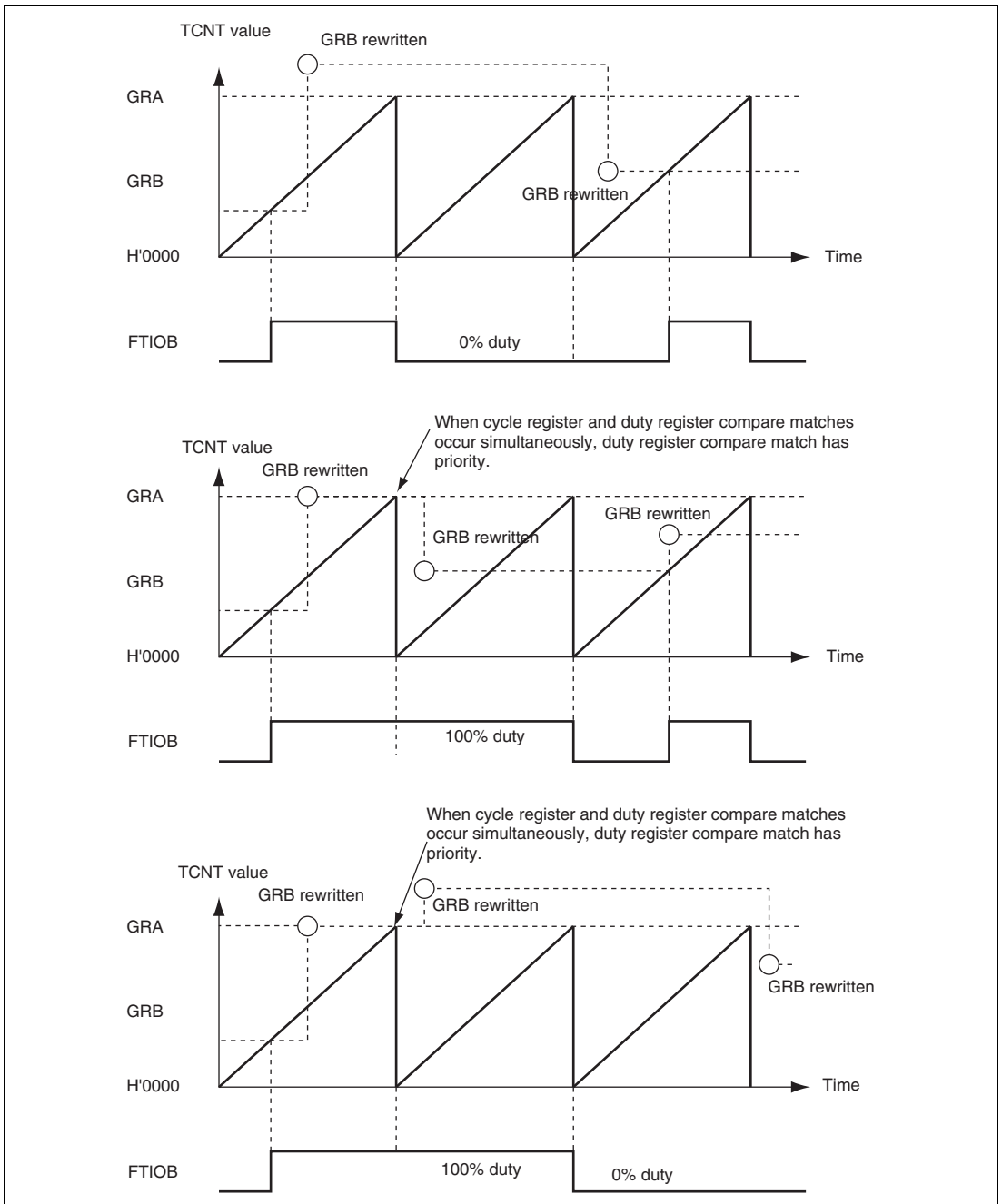
Figure 12.25 Example of PWM Mode Operation (4)
