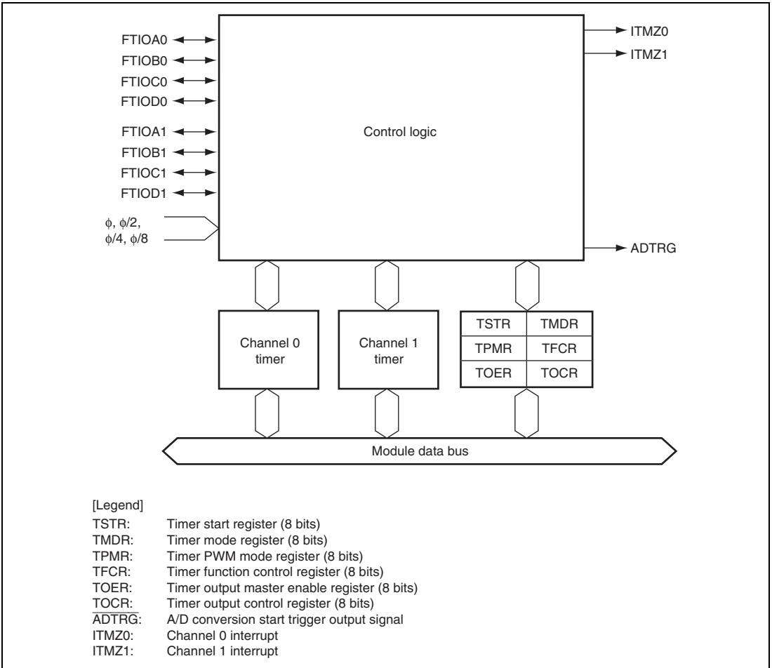
Figure 12.1 Timer Z Block Diagram
