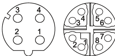
D-coding Mating face acc. to IEC 61076-2-101
