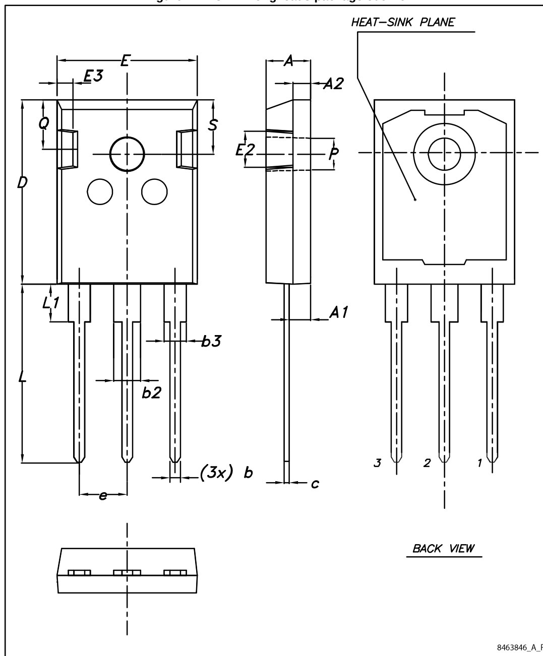
Figure 21: TO-247 long leads package outline
