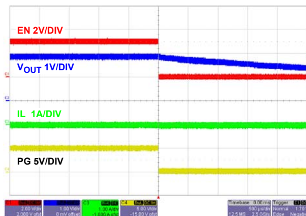
FIGURE 26. SOFT-DISCHARGE SHUTDOWN
