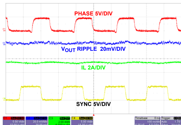
FIGURE 30. STEADY STATE OPERATION AT FULL LOAD (PWM) WITH FREQUENCY = 4MHz
