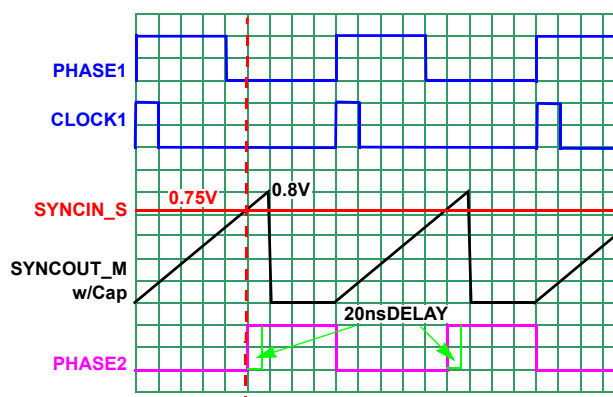
FIGURE 36. SYNCHRONIZATION WAVEFORMS
