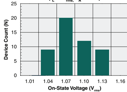
Typical On-State Voltage ( I_L=1\text{A}_{rms} , T_A=25^\circ\text{C} )
