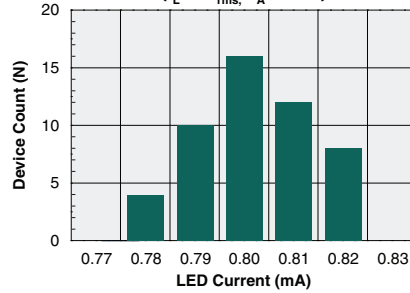
Typical I_F for Switch Operation ( I_L=1\text{A}_{rms} , T_A=25^\circ\text{C} )
