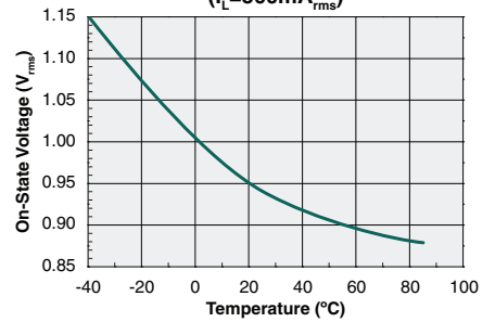
Typical On-State Voltage vs. Temperature ( I_L=500\text{mA}_{rms} )
