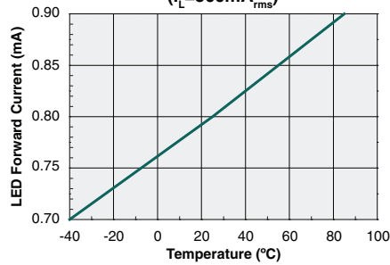
Typical I_F for Switch Operation vs. Temperature ( I_L=500\text{mA}_{rms} )
