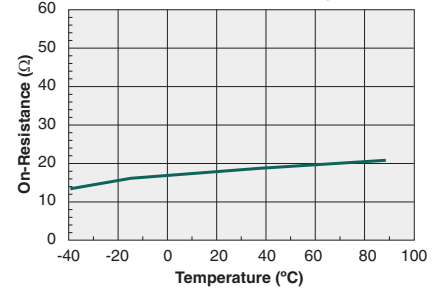
Typical On-Resistance vs. Temperature ( I_F=2\text{mA} , I_L=120\text{mA}_{DC} )
