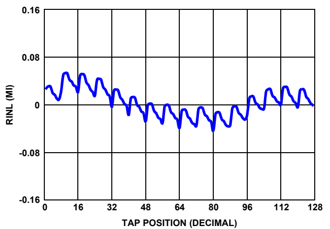
FIGURE 10. 50k RINL vs TAP POSITION, V CC = 5V
