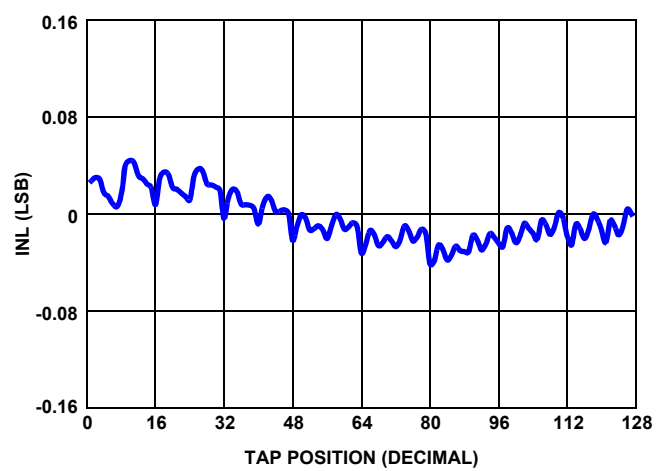
FIGURE 6. 50k INL vs TAP POSITION, V CC = 5V
