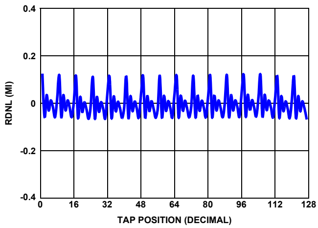
FIGURE 7. 10k RDNL vs TAP POSITION, V CC = 5V
