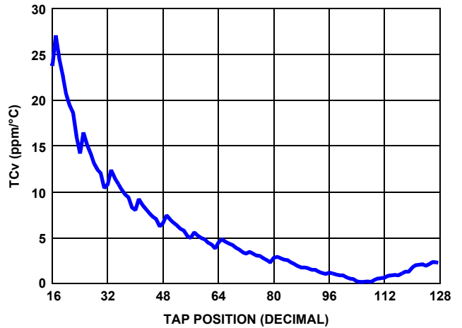
FIGURE 14. 50k TCv vs TAP POSITION
