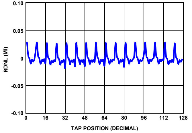
FIGURE 8. 50k RDNL vs TAP POSITION, V CC = 5V
