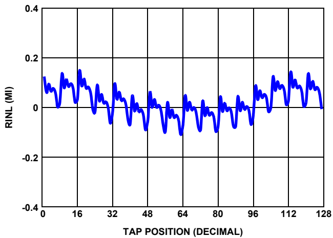
FIGURE 9. 10k RINL vs TAP POSITION, V CC = 5V
