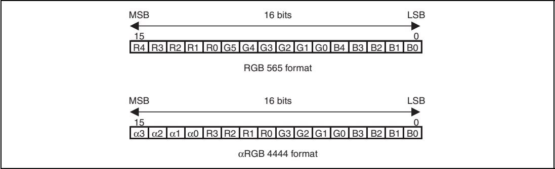
Figure 27.18 Bus Format
