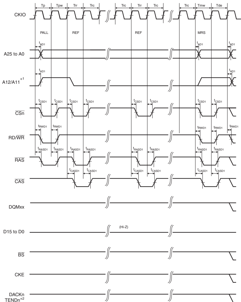
Figure 37.33 Synchronous DRAM Mode Register Write Timing ( WTRP = 1 Cycle)
