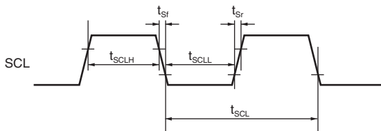
Figure 37.52 (2) Clock Input/Output Timing
