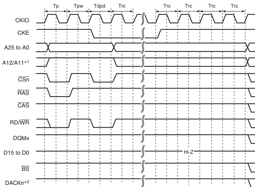
Figure 9.32 Deep Power-Down Mode Transition Timing
