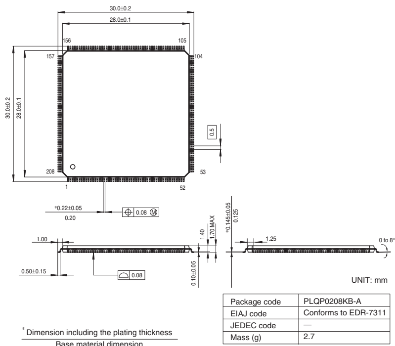
Figure A.2 Package Dimensions of the SH7264
