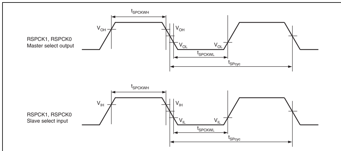
Figure 37.47 Clock Timing
