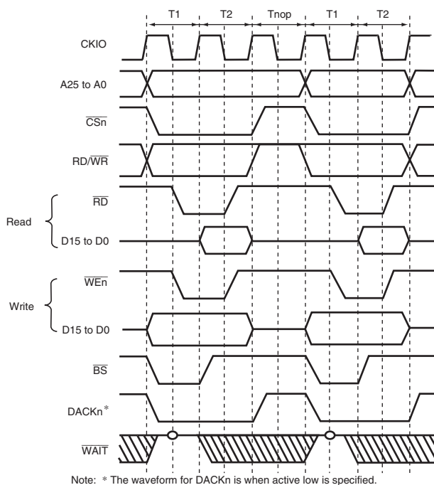
Figure 9.4 Continuous Access to Normal Space (1) Bus Width = 16 Bits, Longword Access, CSnWCR.WM Bit = 0 (Access Wait = 0, Cycle Wait = 0)
