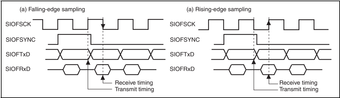
Figure 19.4 Transmit/Receive Timing
