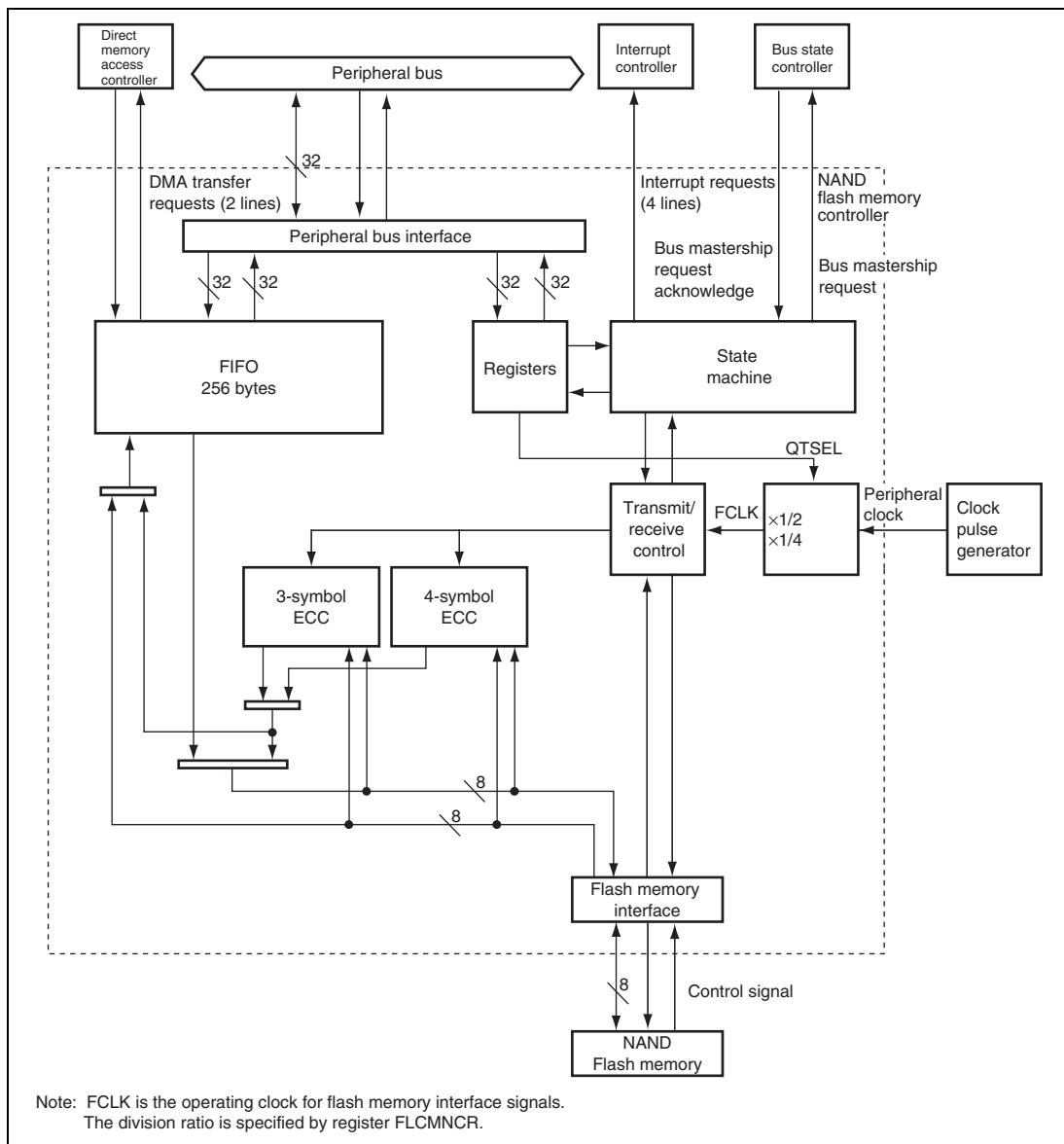
Figure 25.1 Block Diagram
