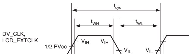
Figure 37.71 DV_CLK and LCD_EXTCLK Clock Input Timing
