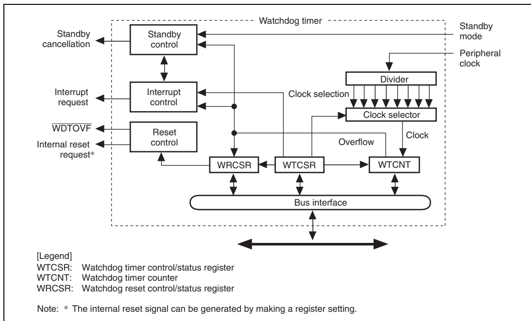
Figure 13.1 Block Diagram
