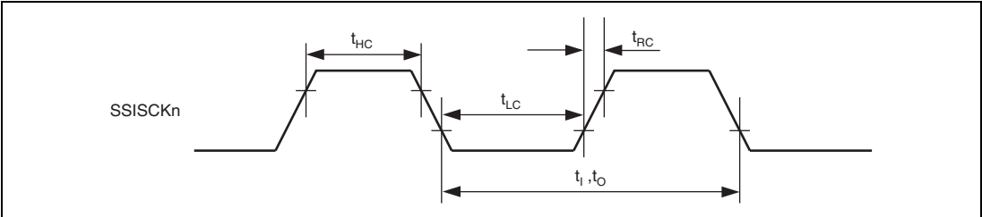
Figure 37.53 Clock Input/Output Timing
