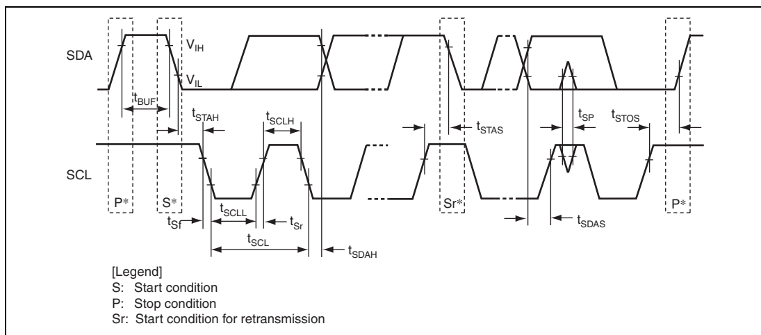
Figure 37.52 (1) Input/Output Timing
