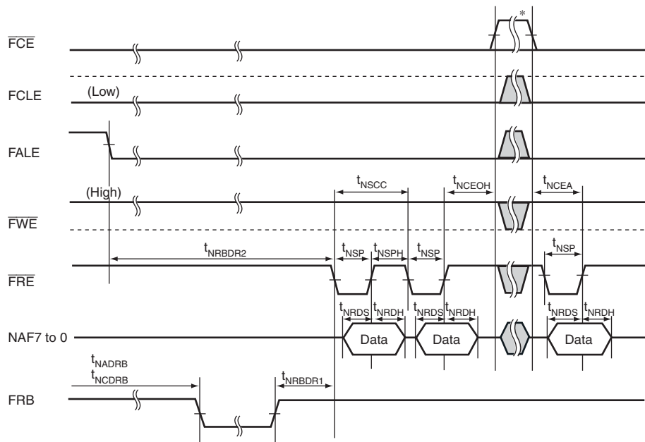
Figure 37.62 NAND Type Flash Memory Data Read Timing
