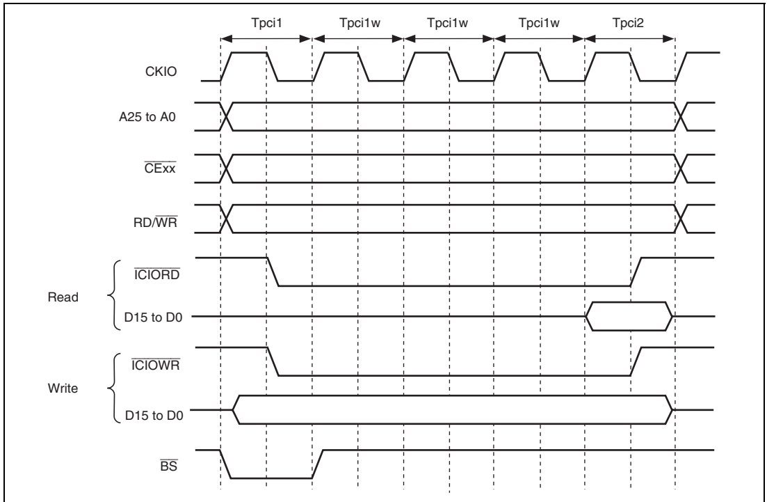
Figure 9.42 Basic Access Timing for PCMCIA I/O Card Interface
