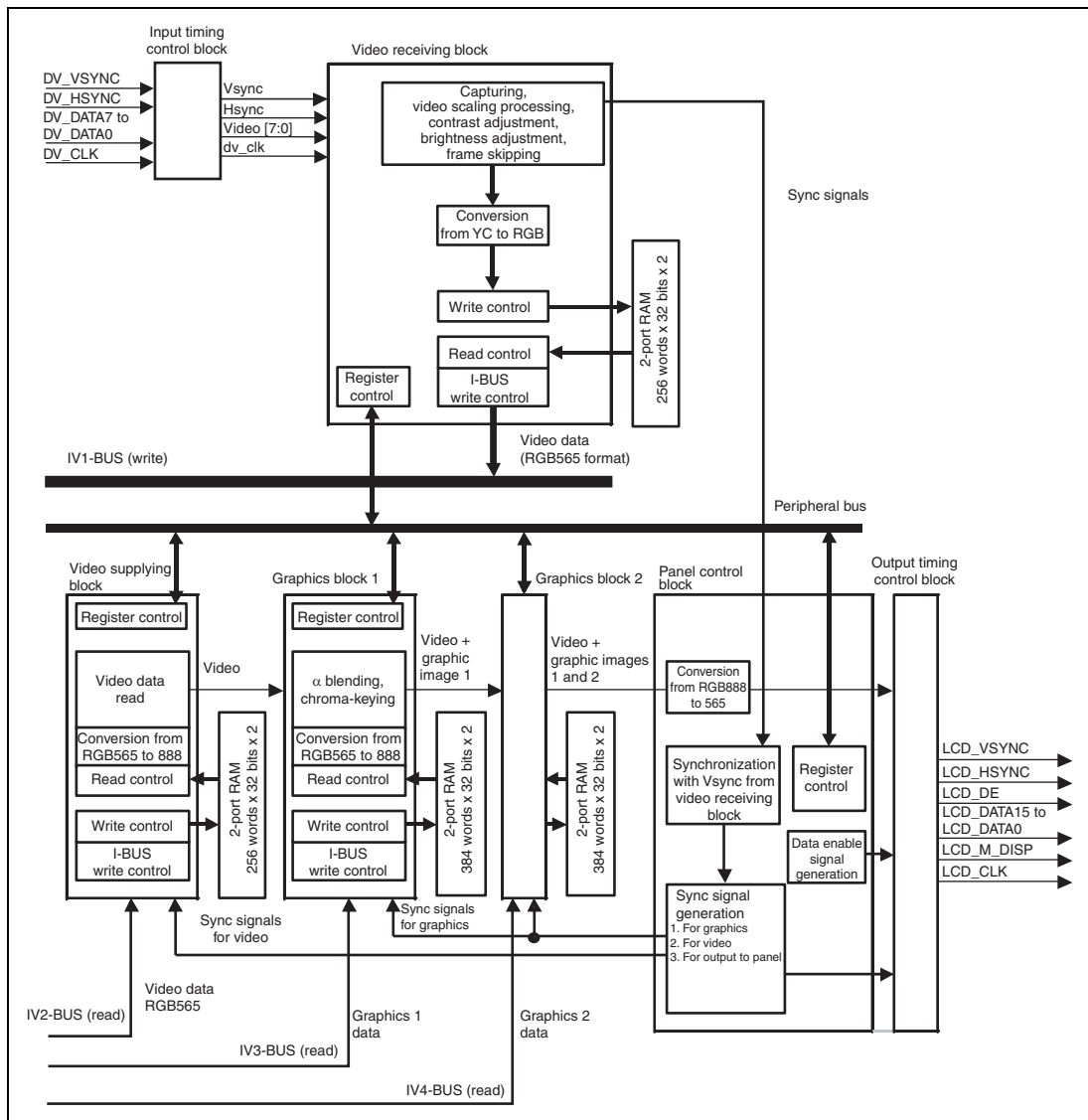
Figure 27.1 Block Diagram
