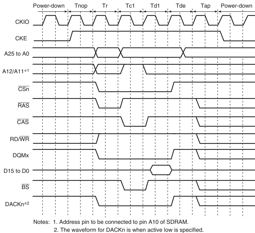
Figure 9.29 Power-Down Mode Access Timing
