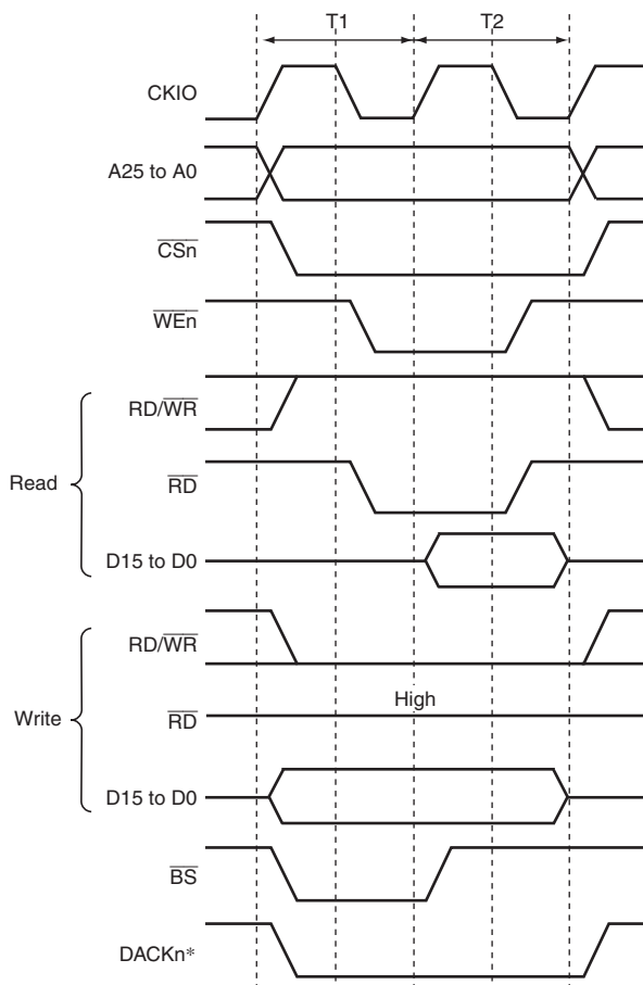
Figure 9.34 Basic Access Timing for SRAM with Byte Selection (BAS = 0)
