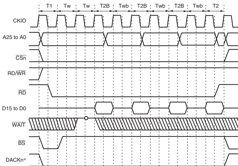
Figure 9.33 Burst ROM Access Timing (Clocked Asynchronous) (Bus Width = 16Bits, 16-Byte Transfer (Number of Burst 4-4), Wait Cycles Inserted in First Access = 2, Wait Cycles Inserted in Second and Subsequent Access Cycles = 1)
