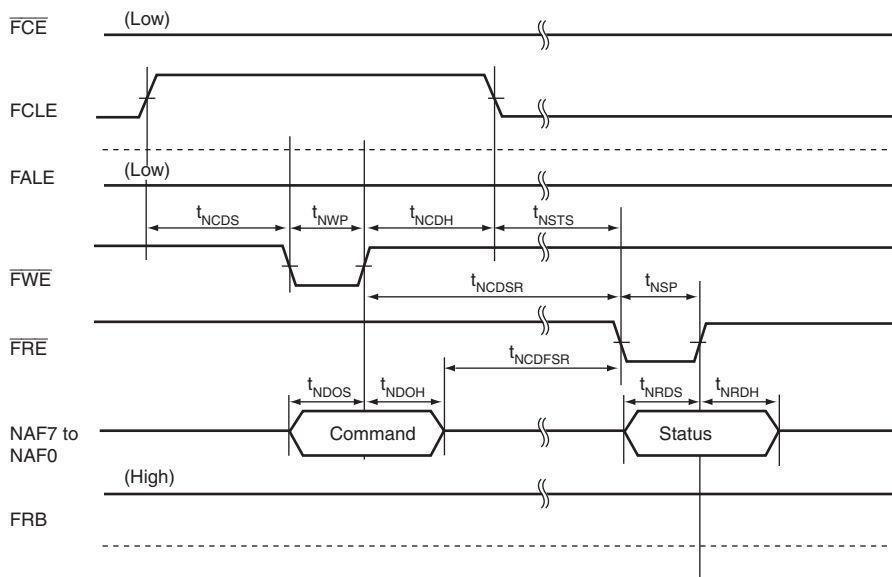
Figure 37.64 NAND Type Flash Memory Status Read Timing
