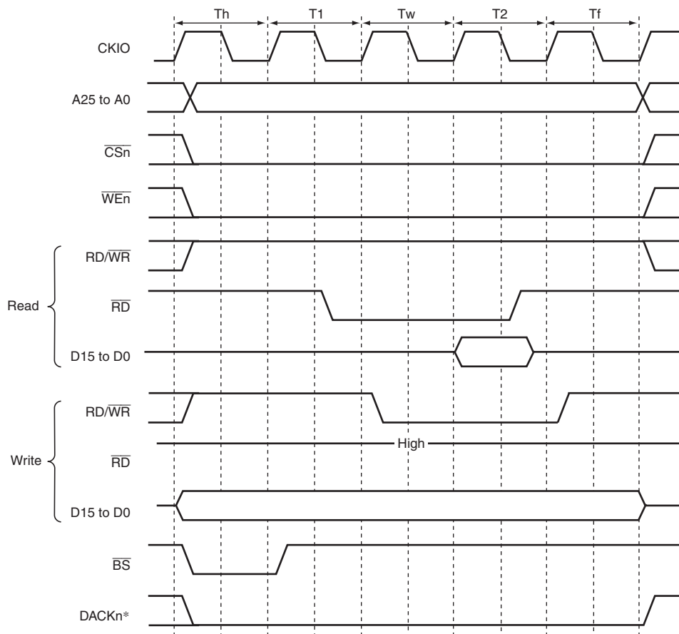
Figure 9.36 Wait Timing for SRAM with Byte Selection (BAS = 1) (SW[1:0] = 01, WR[3:0] = 0001, HW[1:0] = 01)
