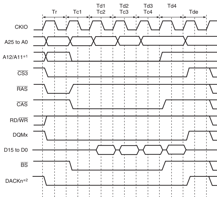
Figure 9.20 Burst Read Timing (Bank Active, Different Bank, CAS Latency 1)
