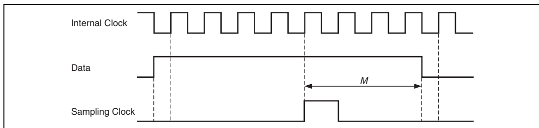
Figure 22.7 Receive Margin
