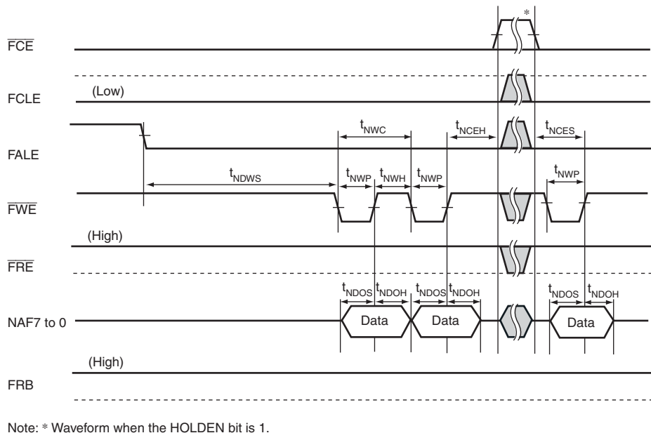
Figure 37.63 NAND Type Flash Memory Data Write Timing
