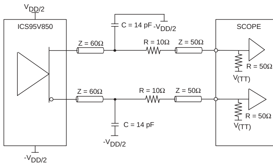
Figure 1. IBIS Model Output Load
