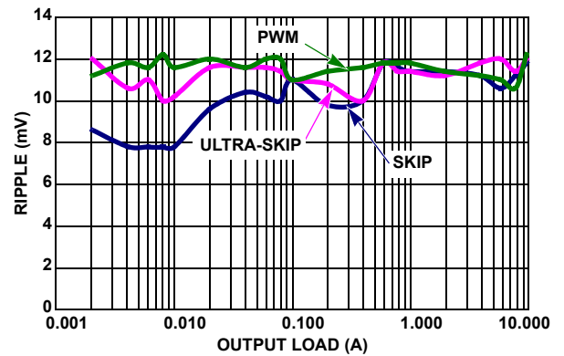
FIGURE 26. V_{OUT2} = 3.3V RIPPLE vs LOAD
