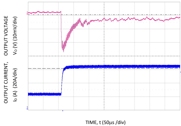
Figure 22. Transient Response to Dynamic Load Change from 25% to 75% at 12Vin, C_o = 25 \times 47\mu F + 8 \times 1000\mu F , R_{TUNE} = 6.81k\Omega
