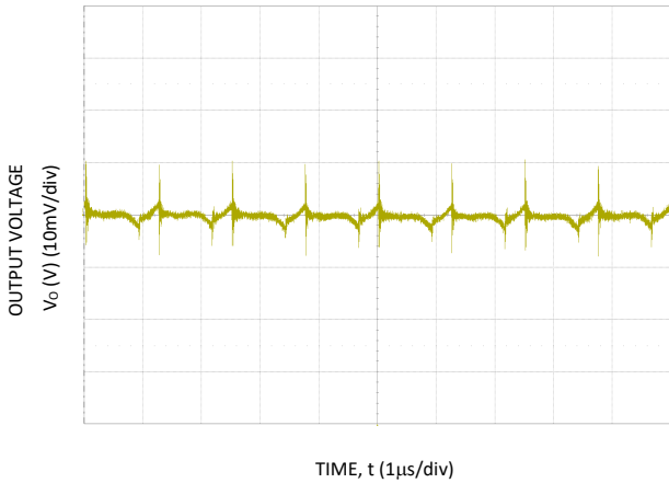
Figure 21. Typical output ripple and noise ( C_o = 6 \times 47\mu F ceramic, V_{IN} = 12V , I_o = I_{o,max} ).
