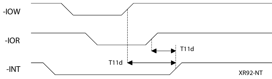
Figure 13: Interrupt Timing
