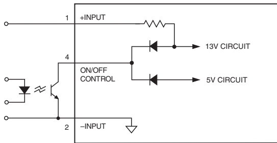
Figure 4. Driving the Positive Logic On/Off Control Pin
