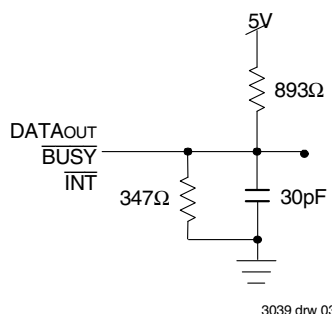
Figure 1. AC Output Test Load
