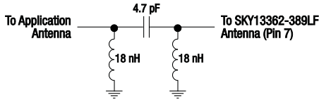
ESD Circuit 1
