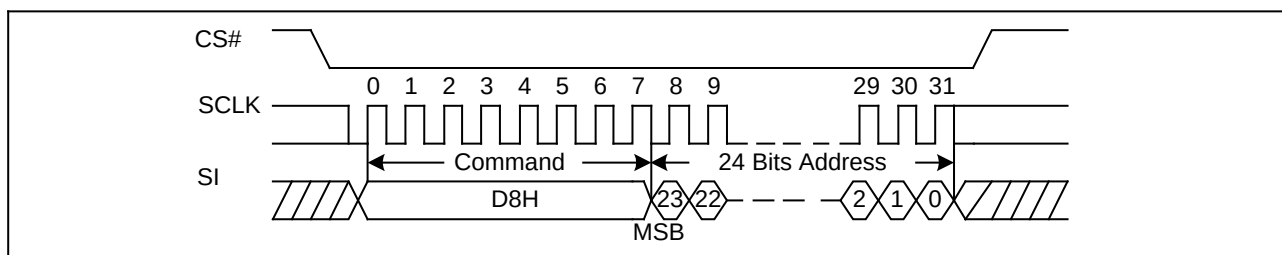
Figure11. 64KB Block Erase Sequence Diagram
