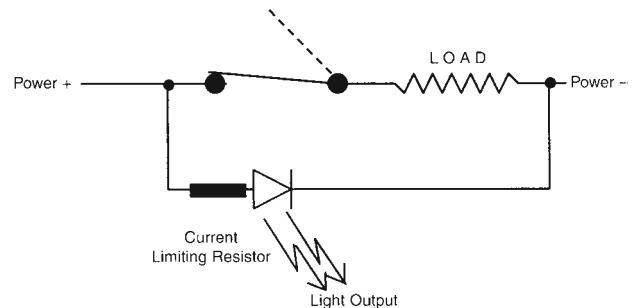
Figure 18. Wiring Diagram 3
