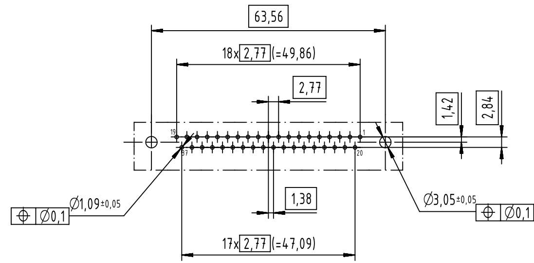
PC-Board layout view component side thickness 1,6
