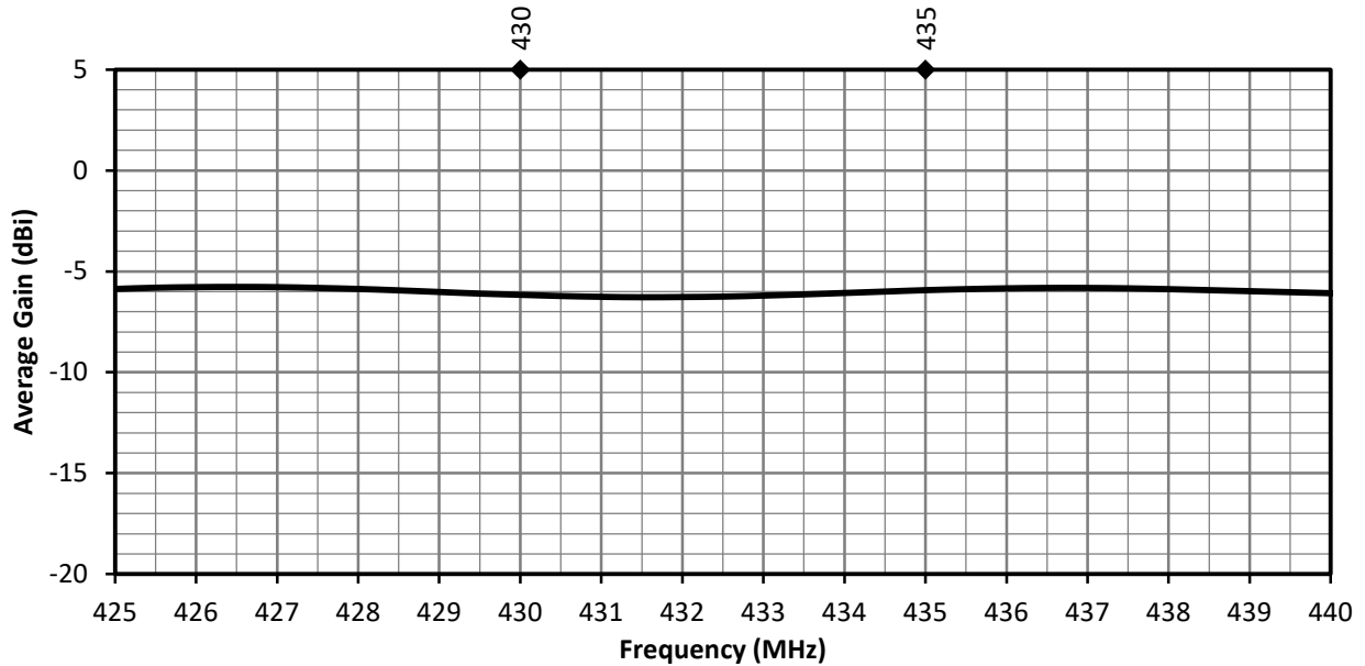
Figure 8. ANT-433-WRT Antenna Average Gain, Free Space
