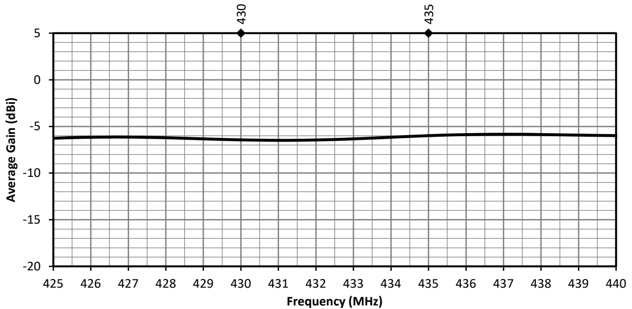
Figure 15. ANT-433-WRT Antenna Average Gain, at Center of Ground Plane
