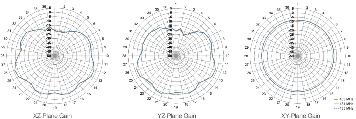
Figure 10. ANT-433-WRT Radiation Patterns, Free Space
