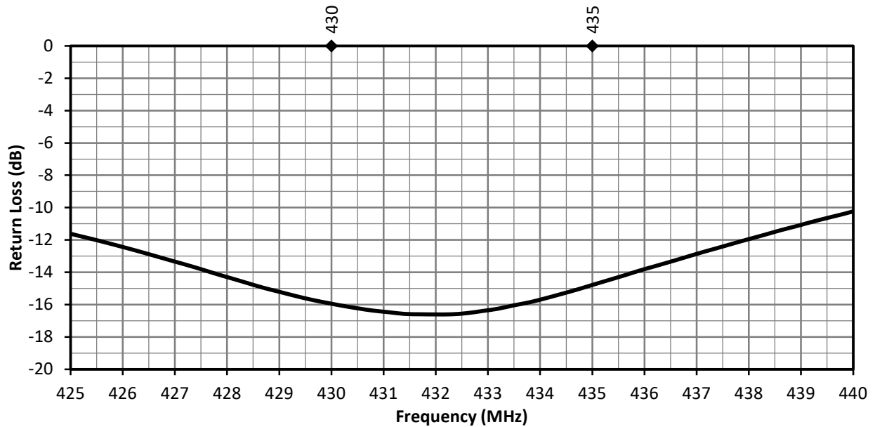
Figure 6. ANT-433-WRT Return Loss, Free Space
