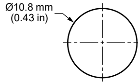
Figure 2. ANT-433-WRT Series Antenna Recommended Enclosure Mounting Dimensions
