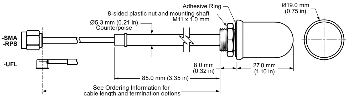
Figure 1. ANT-433-WRT Antenna Dimensions
