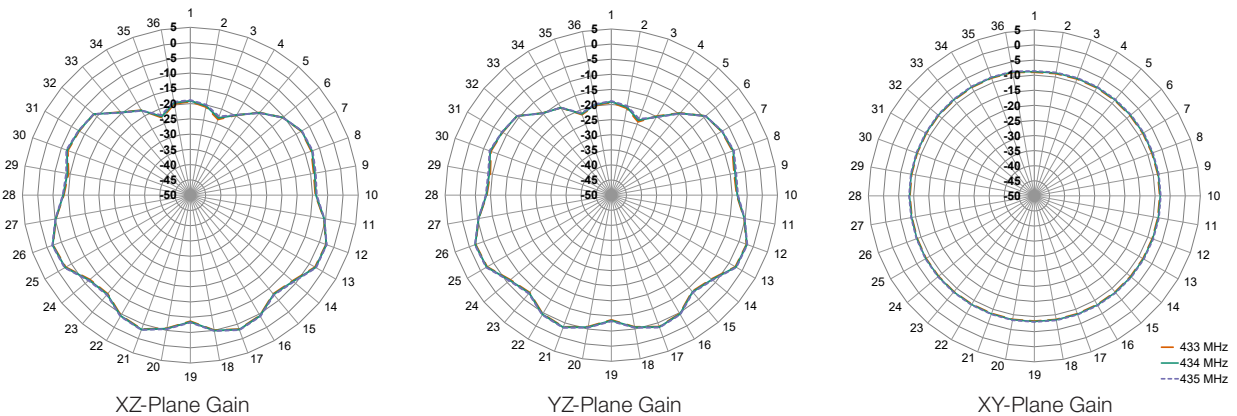
Figure 17. ANT-433-WRT Radiation Patterns, Center of Ground Plane
