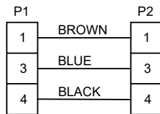
WIRING DIAGRAM
