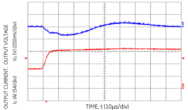
Figure 12. Transient Response to Dynamic Load Change from 50% to 100% of full load (Vo = 5.0 Vdc, Cext = 2x150 µF Polymer Capacitors).
