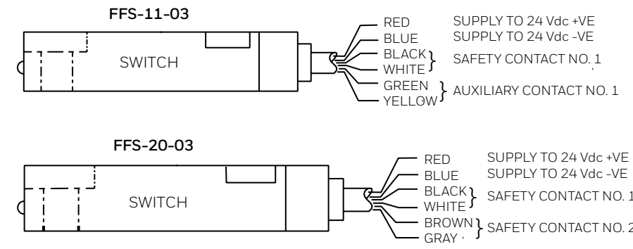
Figure 3. FFS Series Connections
