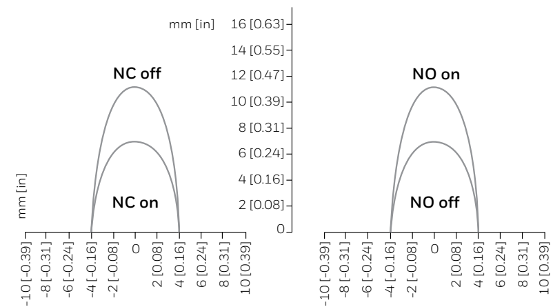
Figure 1. FFS Series Distance
