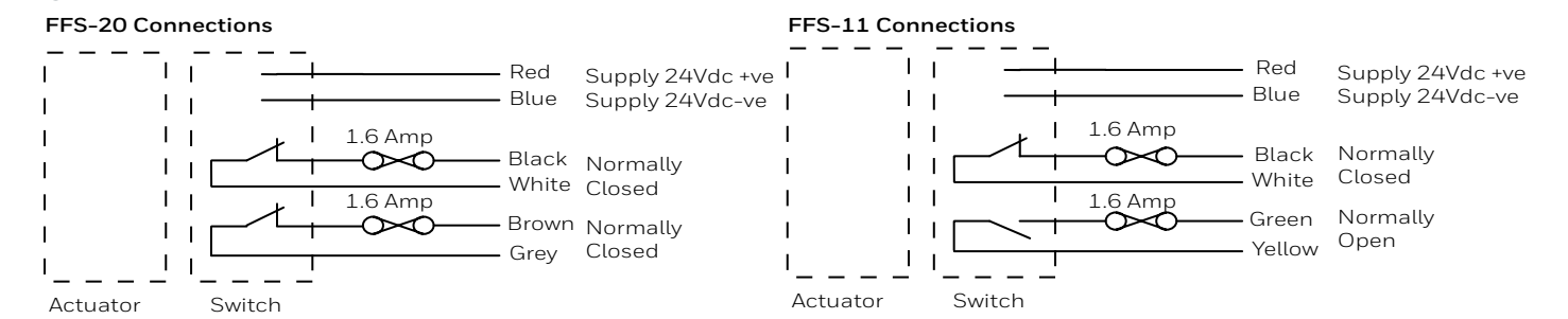
Figure 2. FFS Series Contacts
