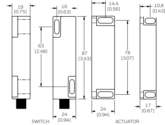
Figure 5. FFS Series Dimensions
