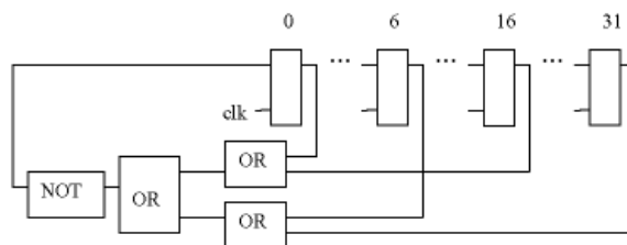
Figure 2–9. Linear Feedback Shift Register Design
