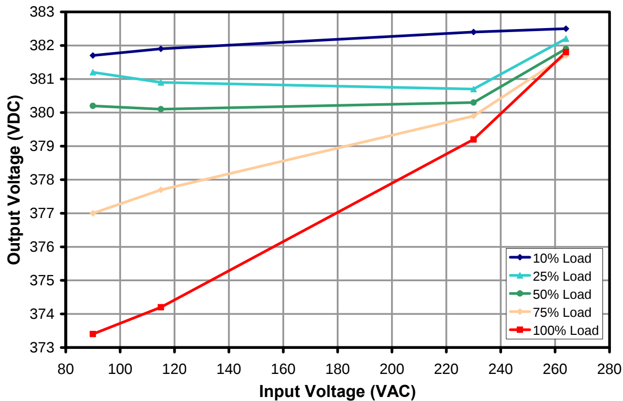
Figure 18 – Line Regulation.
