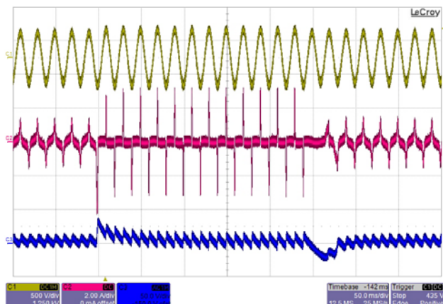
Figure 59 – Line Surge 264 VAC, 50% Load. Upper: V_{IN} , 500 V / div. Middle: I_{IN} , 2 A / div. Lower: V_{OUT} (AC Coupled), 50 V / div. , 50 ms / div.
