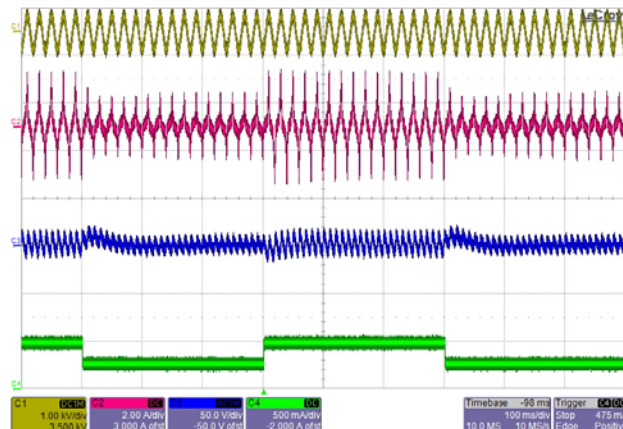
Figure 46 – Transient Response, 264 VAC, 50-100-50% Load Step. Upper: V_{IN} , 1 kV / div. Second: I_{IN} , 2 A / div. Third: V_{OUT} (AC Coupled), 50 V / div. Lower: I_{LOAD} 500 mA, 100 ms / div.
