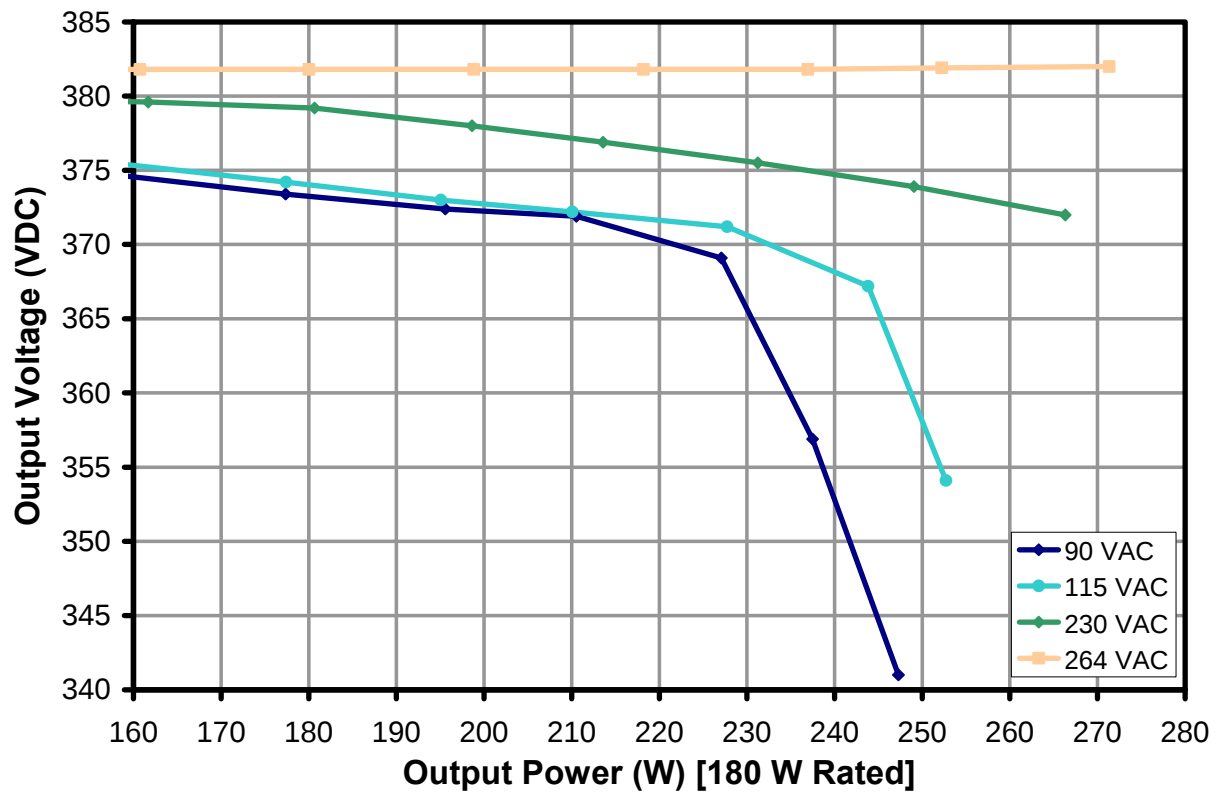
Figure 19 – Overload Regulation.
