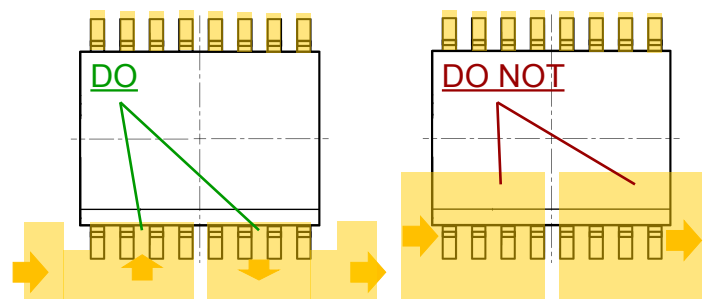
Figure 7: Best Practice Layout Techniques for Current Traces
