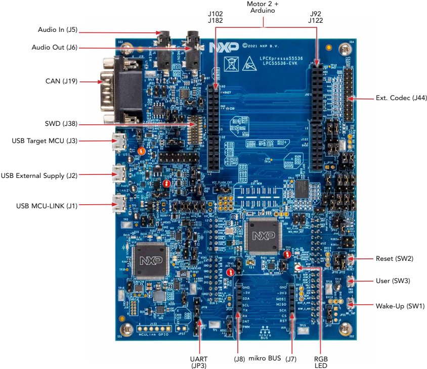
Figure 1: LPC5536-EVK Pin-Out
