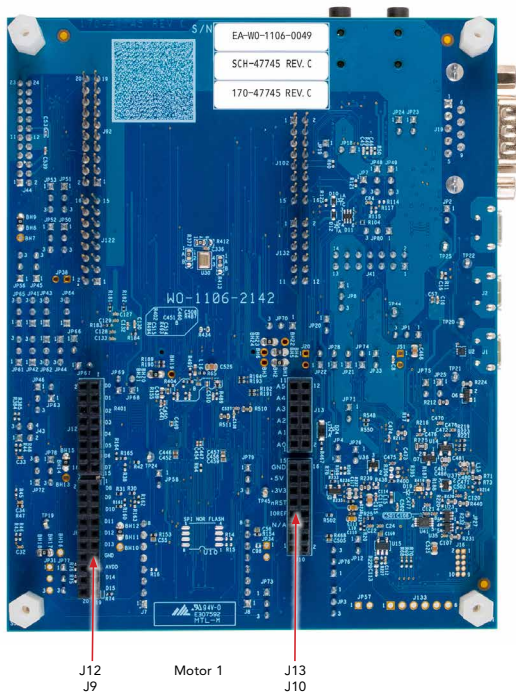
Figure 2: LPC5536-EVK Pin-Out
