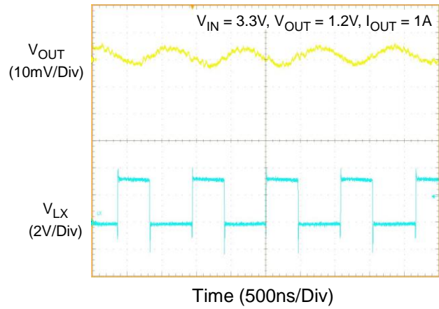
Voltage Ripple
