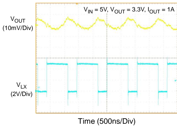
Voltage Ripple
