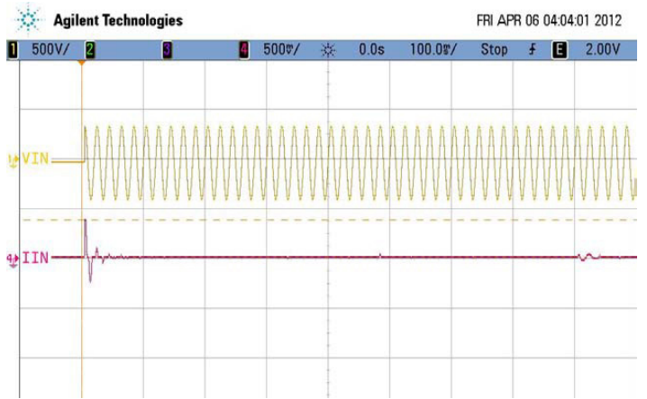
Inrush Current
