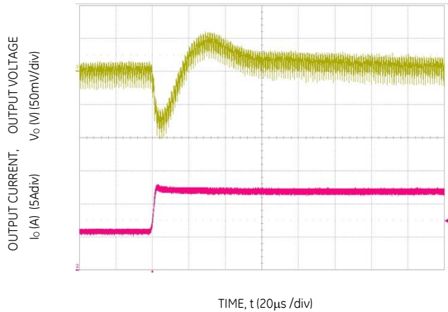
Figure 28. Transient Response to Dynamic Load Change from 50% to 100% at 12V in , C out = 2x47μF+1x330μF, C Tune =2700pF & R Tune =300Ω
