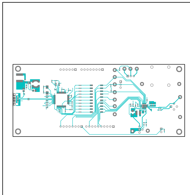
MAX22514 EV Kit PCB Layout—Top
