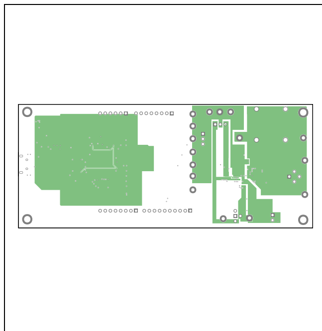
MAX22514 EV Kit PCB Layout—Layer 3
