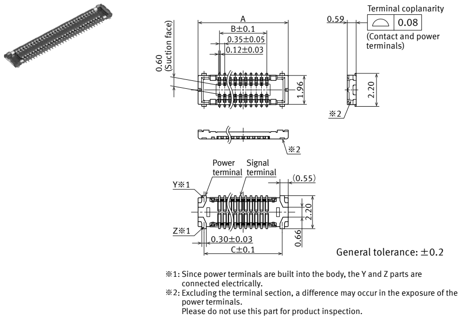
Dimension table
