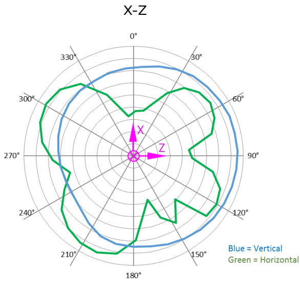
Figure 11: X-Z plane antenna pattern
