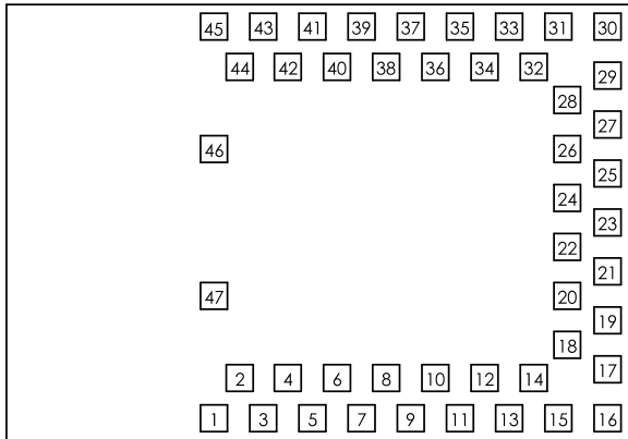
Figure 2: BMD-300 Pin assignment (top view)
