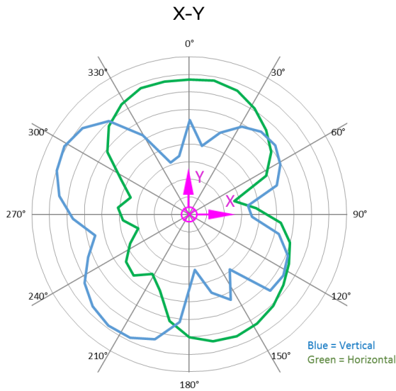
Figure 10: X-Y plane antenna pattern
