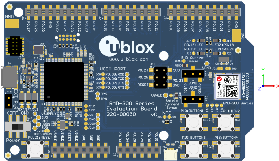
Figure 9: BMD-300 evaluation kit X-Y-Z orientation
