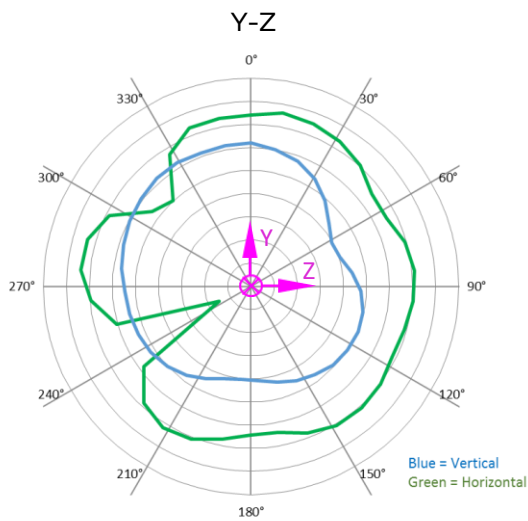
Figure 12: Y-Z plane antenna pattern
