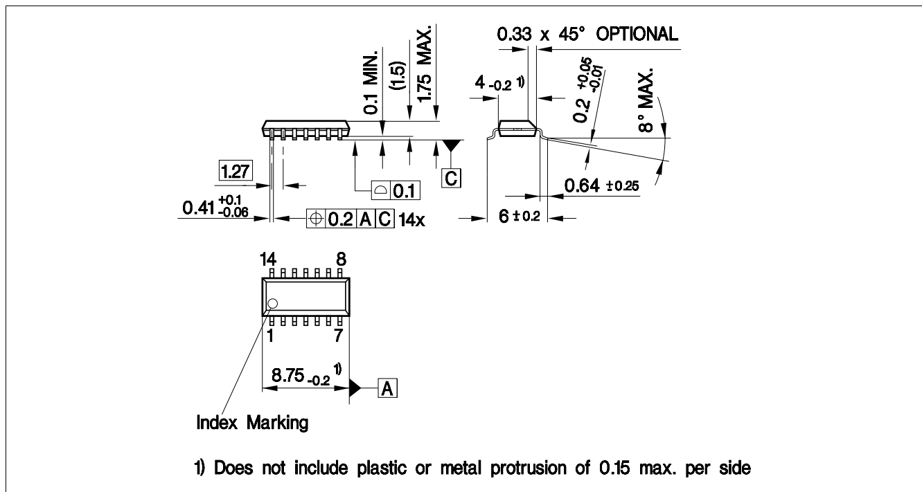
Figure 10 PG-DSO-14 1)
