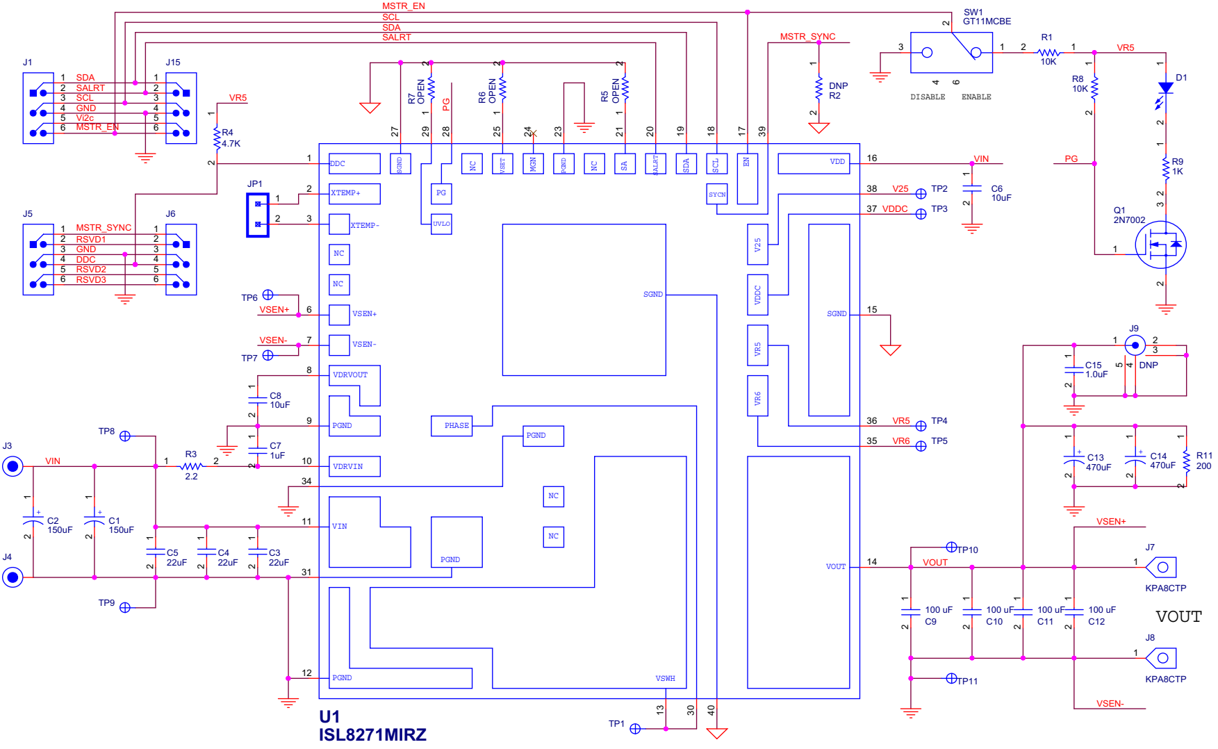
FIGURE 2. APPLICATION CIRCUIT
