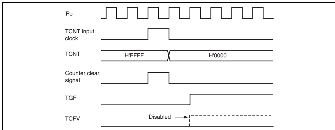
Figure 12.123 Contention between Overflow and Counter Clearing
