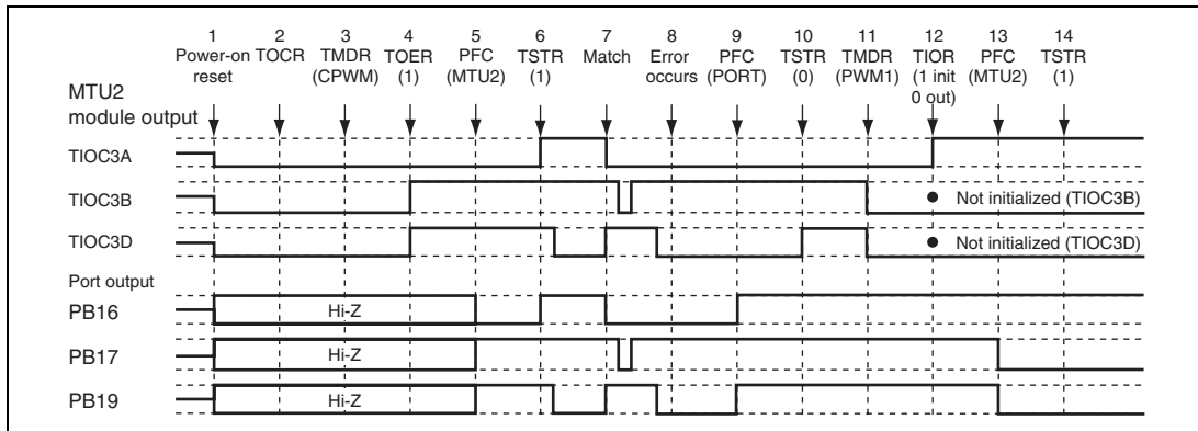
Figure 12.148 Error Occurrence in Complementary PWM Mode, Recovery in PWM Mode 1
