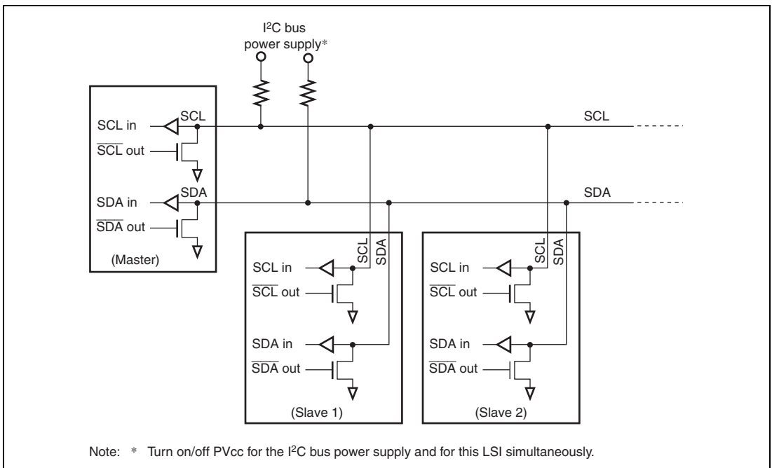
Figure 17.2 External Circuit Connections of I/O Pins
