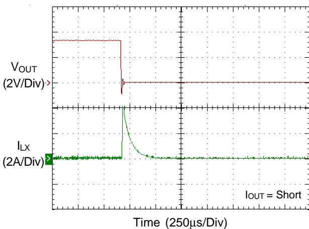
Figure 6. Latch-Off Mode Under Voltage Protection
