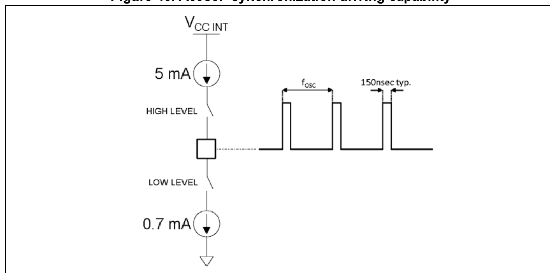
Figure 46. A6985F synchronization driving capability
