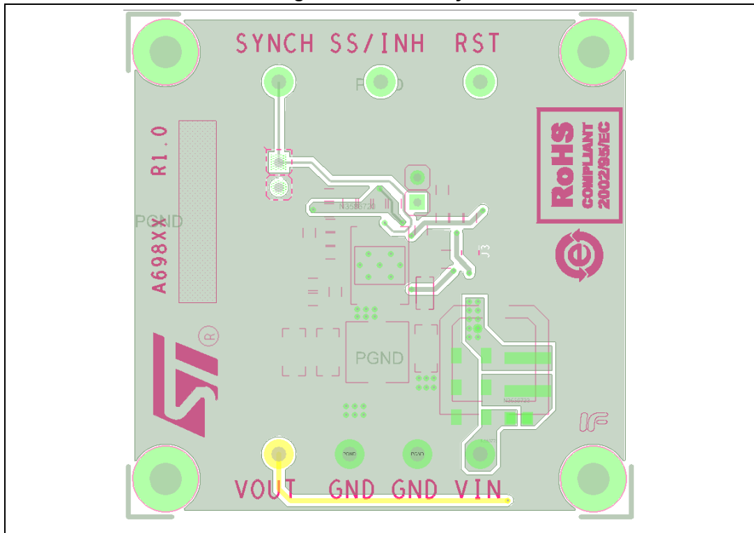
Figure 51. Bottom layer
