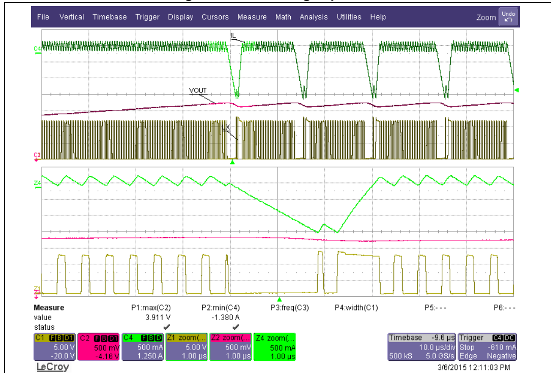
Figure 34. Overtoltage operation
