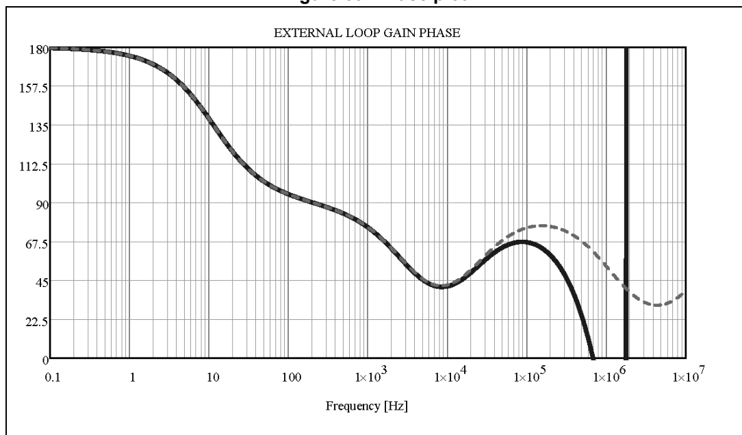
Figure 39. Phase plot
