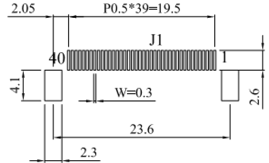
DETAIL J1 SCALE 2/1
