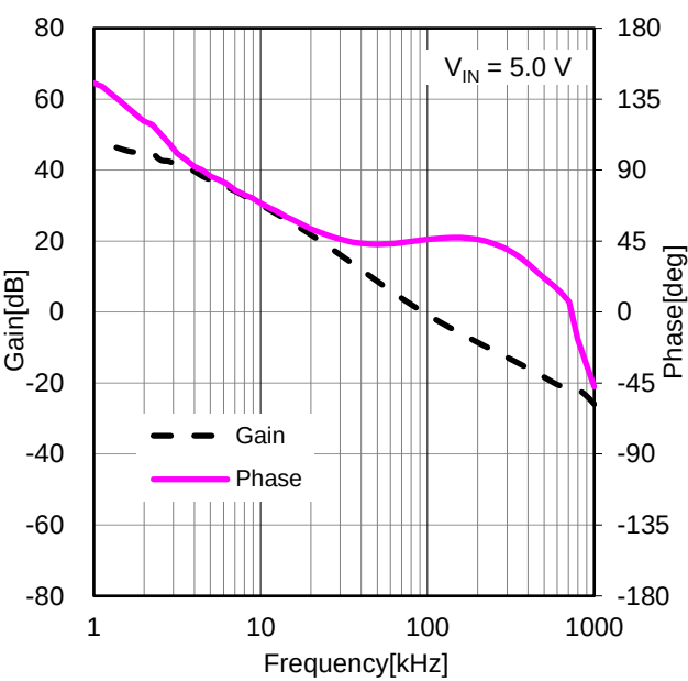
Figure 52. Frequency Characteristics ( I_{OUT} = 2\text{ A} )
