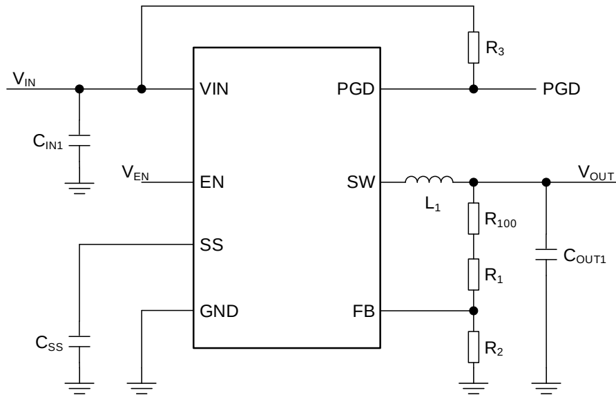
Figure 25. Typical Application
