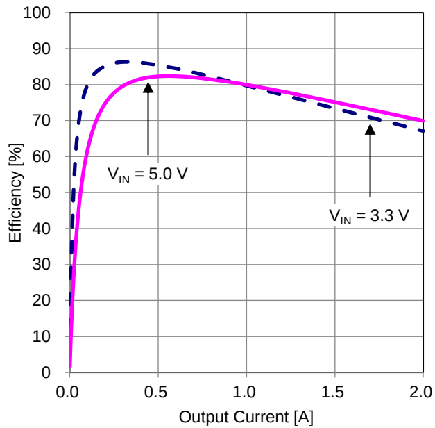
Figure 31. Efficiency vs Output Current
