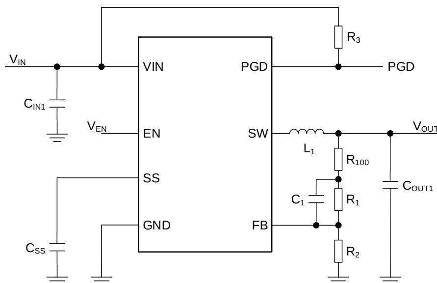
Figure 35. Reference Circuit 2
