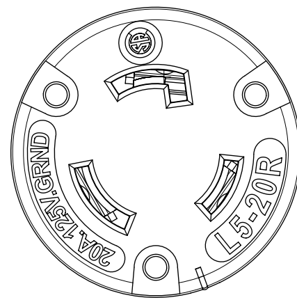
FACE VIEW
