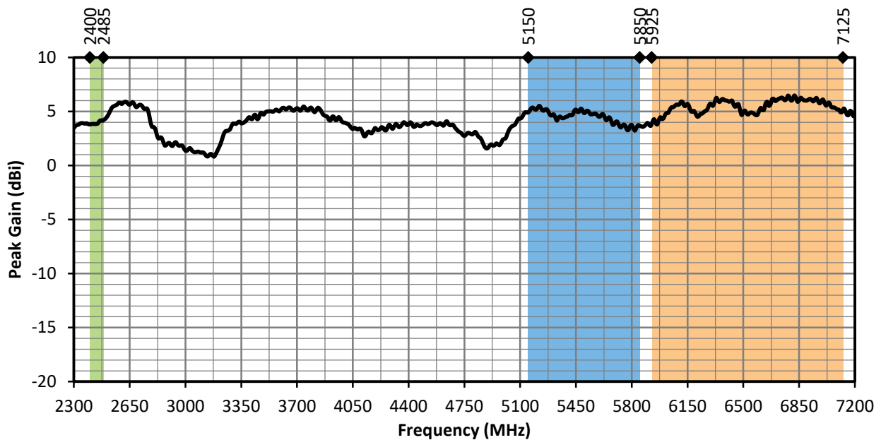
Figure 13. ANT-W63-IPW2-NP Antenna Peak Gain, Center of Ground Plane
