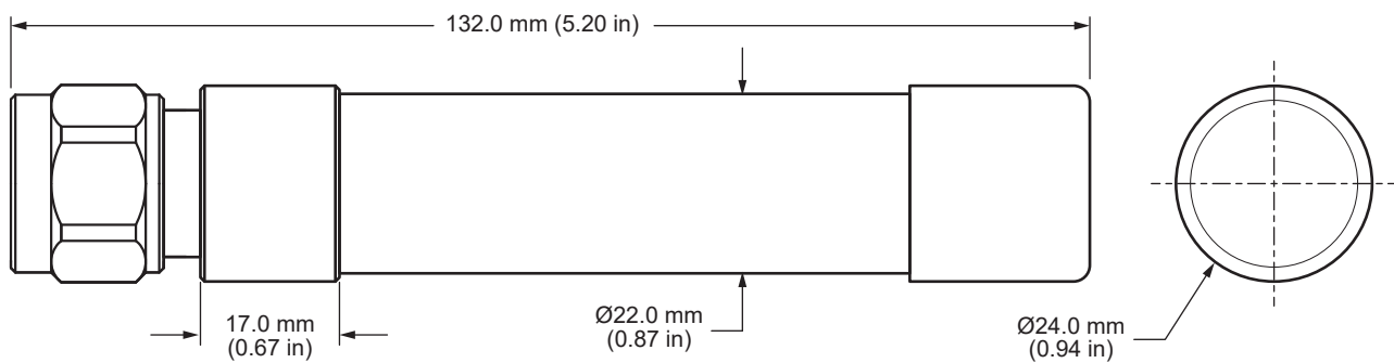
Figure 1. ANT-W63-IPW2-NP Antenna Dimensions
