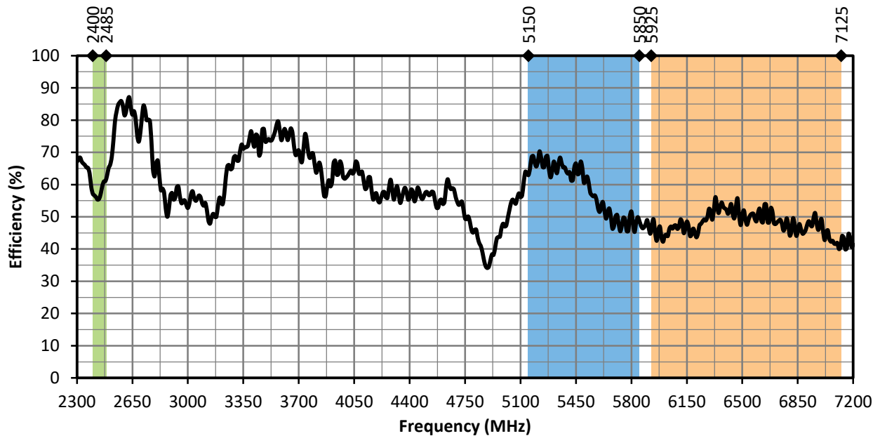
Figure 8. ANT-W63-IPW2-NP Series Antenna Radiation Efficiency, Free Space
