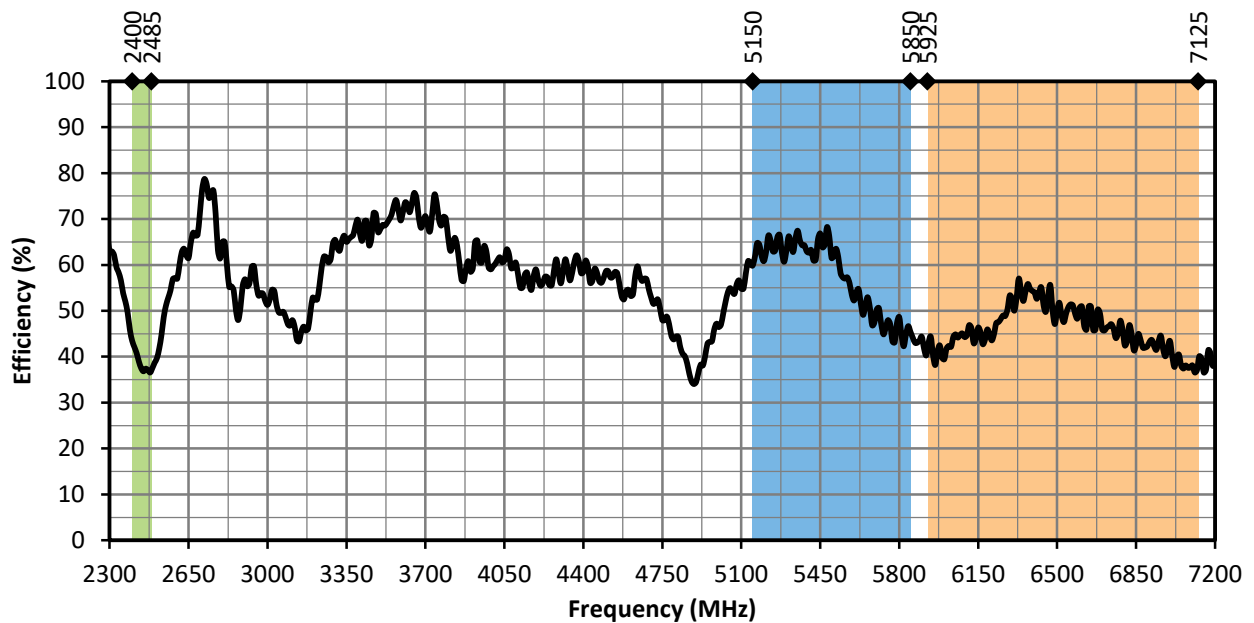
Figure 15. ANT-W63-IPW2-NP Antenna Radiation Efficiency, Center of Ground Plane
