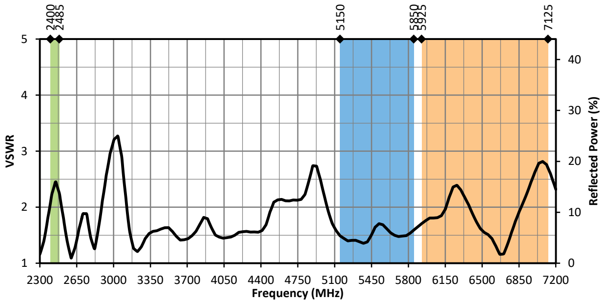
Figure 4. ANT-W63-IPW2-NP VSWR, Free Space
