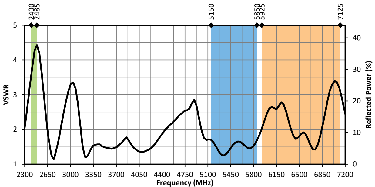
Figure 11. ANT-W63-IPW2-NP Antenna VSWR, Center of Ground Plane
