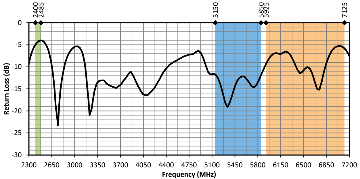
Figure 12. ANT-W63-IPW2-NP Antenna Return Loss, Center of Ground Plane
