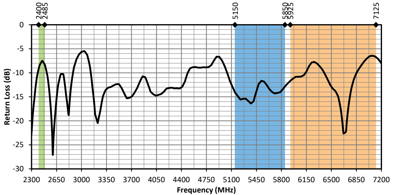
Figure 5. ANT-W63-IPW2-NP Return Loss, Free Space
