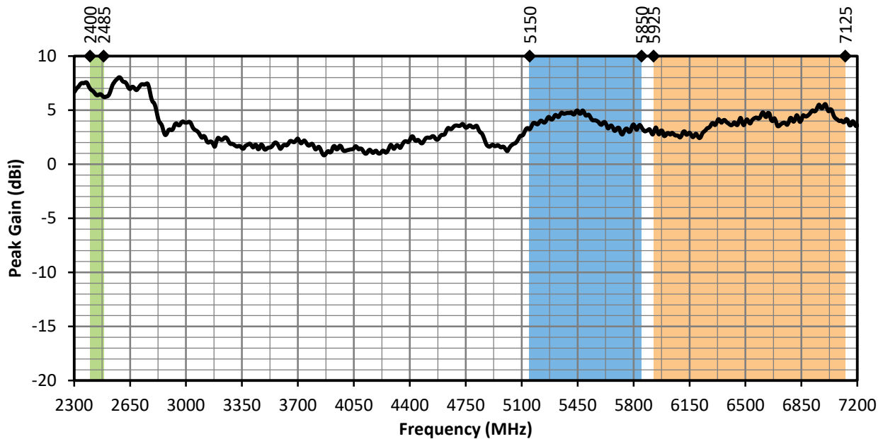
Figure 6. ANT-W63-IPW2-NP Peak Gain, Free Space
