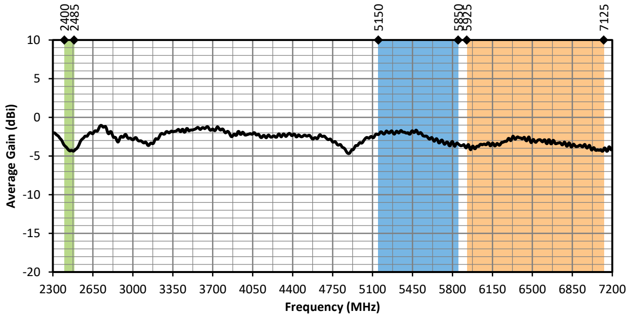
Figure 14. ANT-W63-IPW2-NP Antenna Average Gain, Center of Ground Plane
