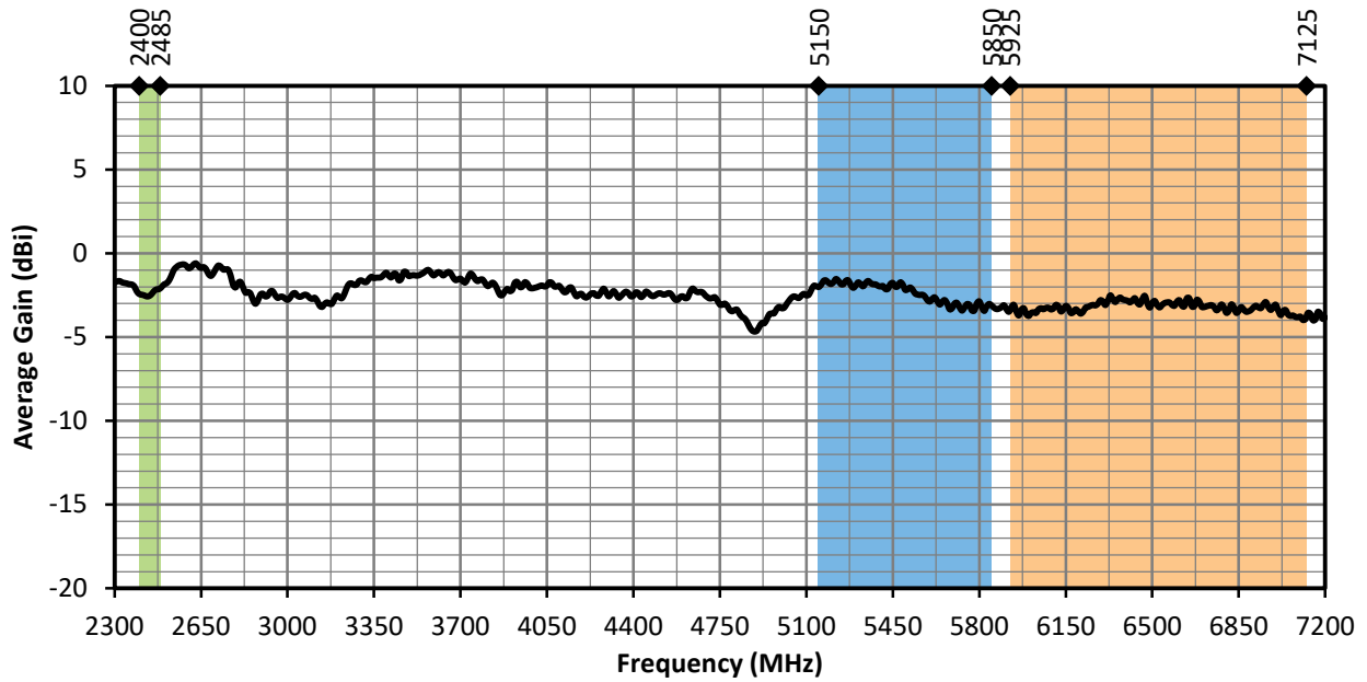
Figure 7. ANT-W63-IPW2-NP Antenna Average Gain, Free Space
