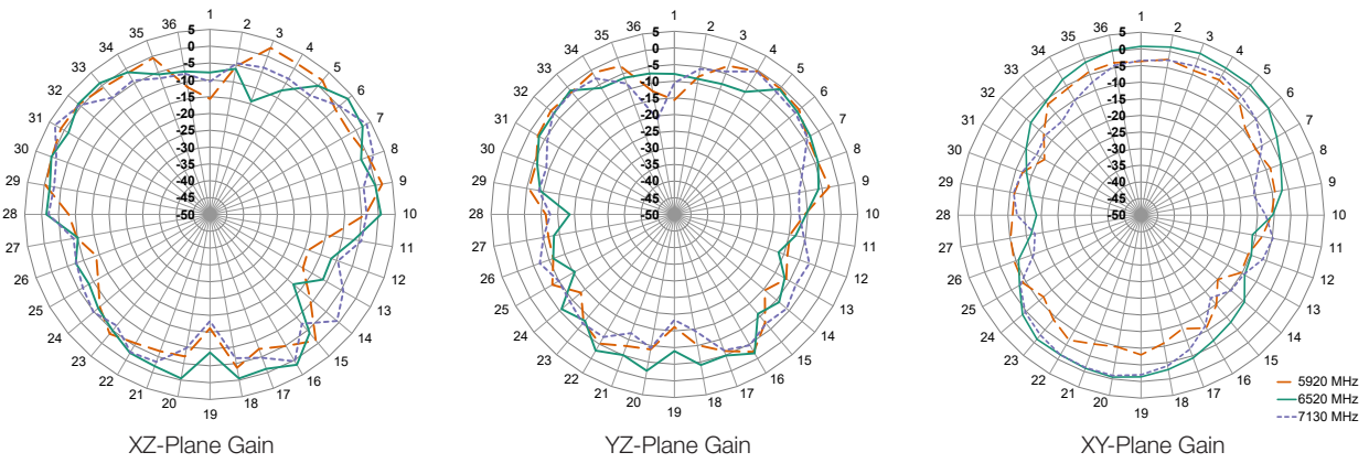
Figure 9. ANT-W63-IPW2-NP Antenna Radiation Patterns, Free Space
