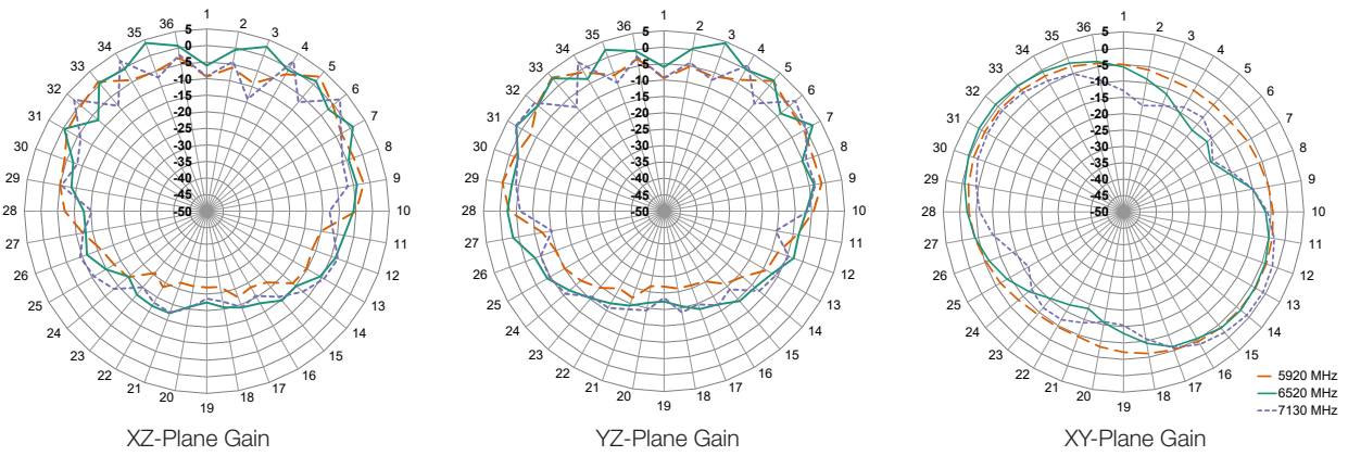
Figure 16. Radiation Patterns for the ANT-W63-IPW2-NP Antenna, Center of Ground Plane
