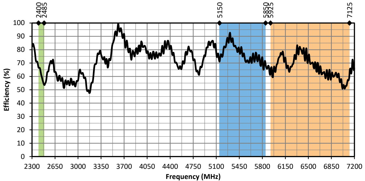
Figure 8. ANT-W63-IPW1-NP Antenna Radiation Efficiency, Free Space
