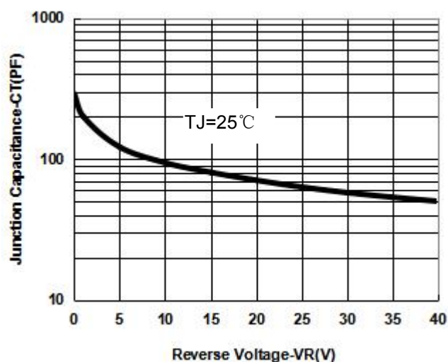
Fig.1-Typical Junction Capacitance
