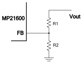
Figure 10: Feedback Network
