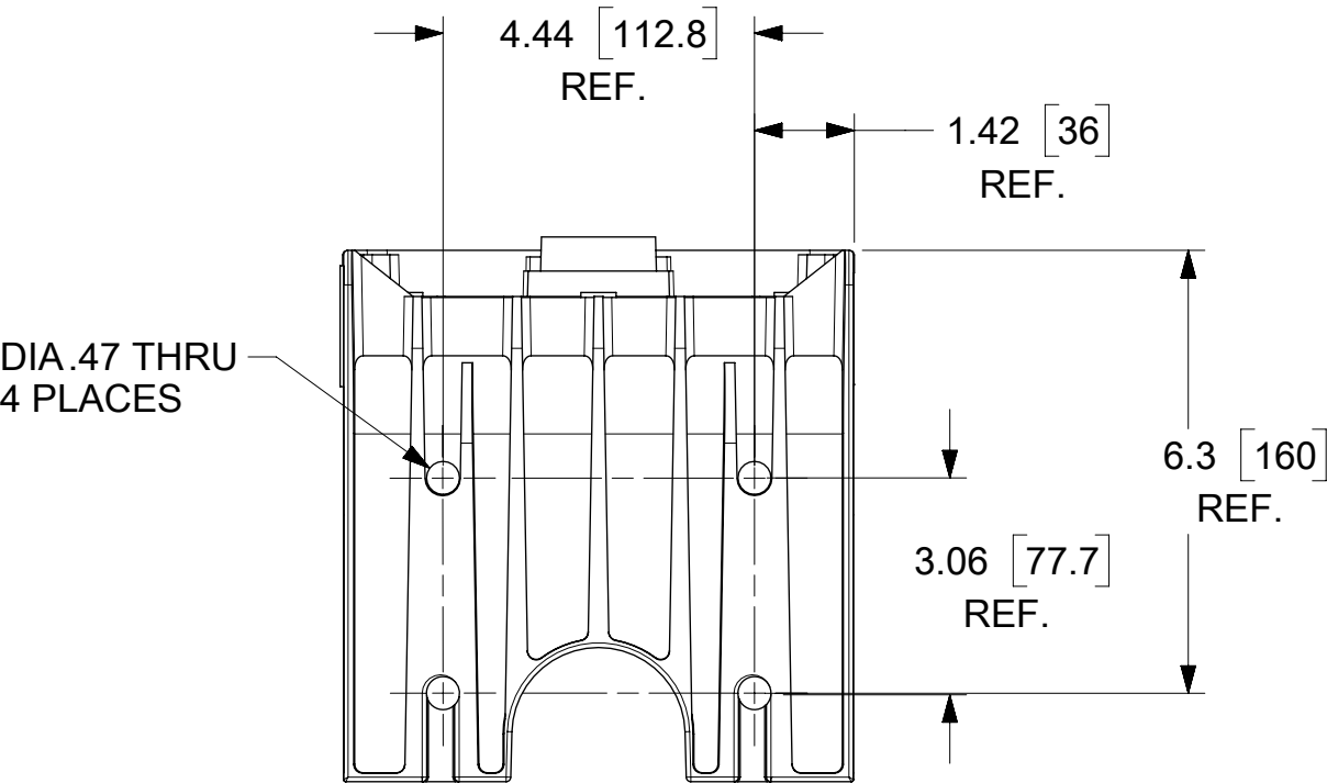
BOTTOM VIEW
