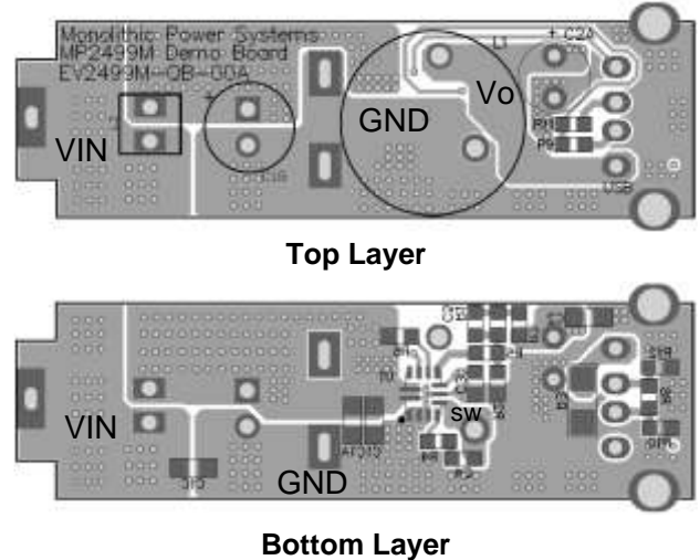
Figure 9: Recommended PCB Layout
