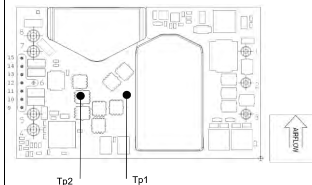
Base plate (Bottom view)
