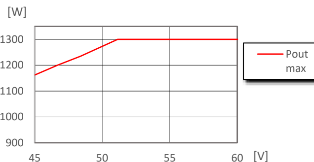
Available output power vs. input voltage, T_{P1} = +25^{\circ}\text{C}
