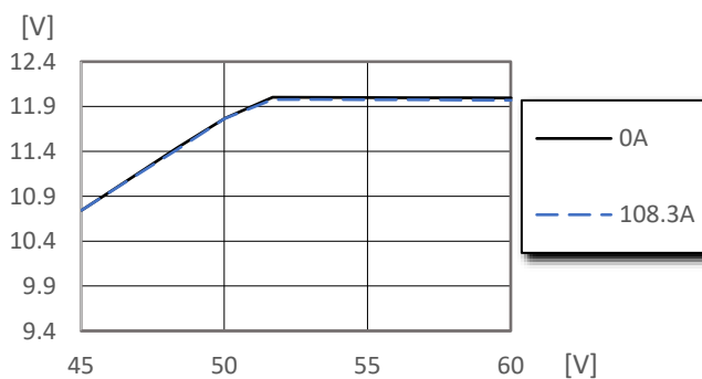
Output voltage vs. input voltage at T_{P1} = +25^{\circ}\text{C}
