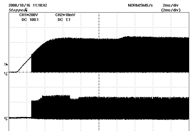
Figure 17 – 265 VAC Input and Full Load. Upper: V_{DRAIN} , 200 V, 2 ms / div. Lower: I_{DRAIN} , 0.2 A / div.
