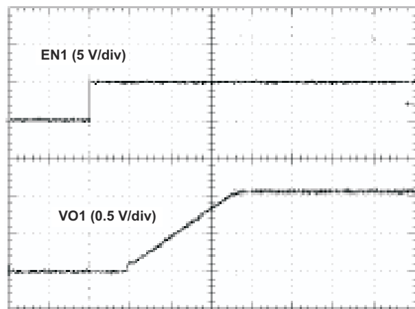
Figure 4-2. 1.05-V Start-Up Waveforms
