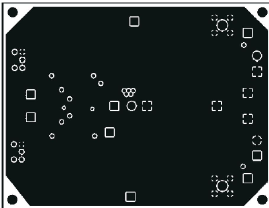
Figure 6-5. Inner Layer 2
