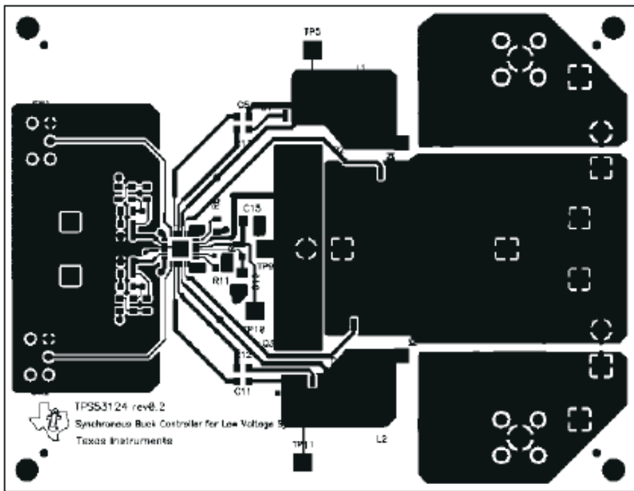
Figure 6-3. Top Layer
