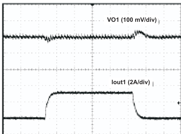
Figure 4-4. 1.05-V Load Transient Response
