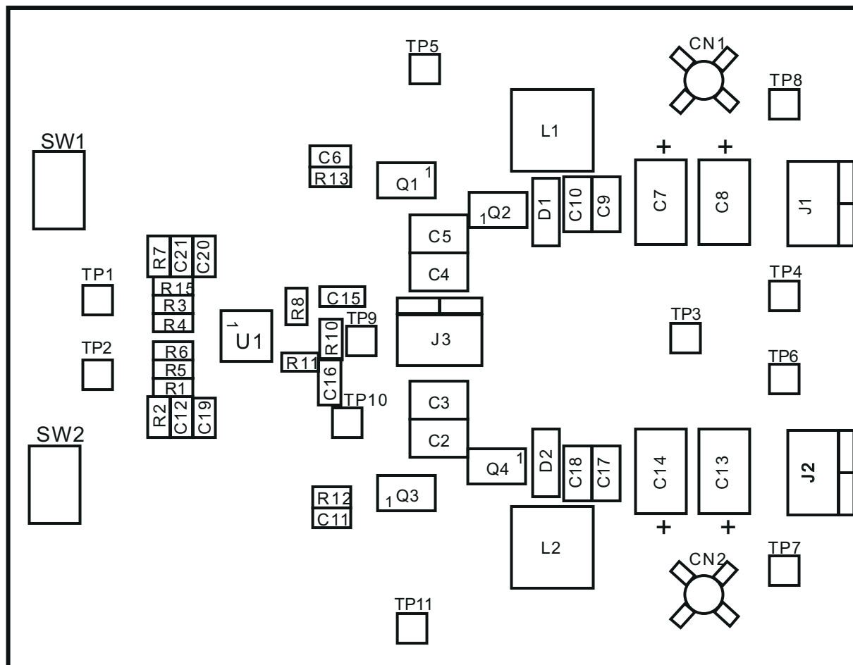
Figure 6-1. Top Assembly
