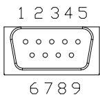
D-SUB FACE VIEW
